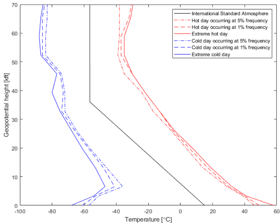
Figure 5: Typical outside ambient temperature design conditions for aircraft based on the international standard atmosphere and the U.S. military handbook, MIL-HNDB-310 [25].
