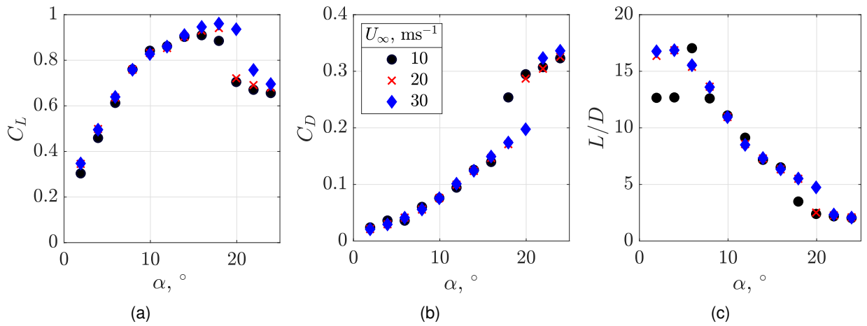
Figure 9 – Wing model C_L , C_D , and L/D measured at three wind-speeds.
