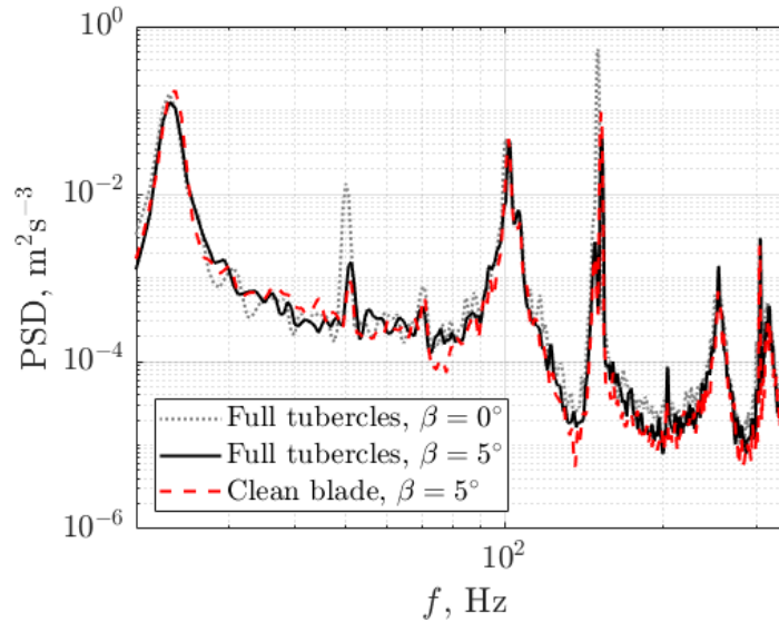
Figure 15 – Power spectral density of the acceleration measured on the wing at U_\infty = 20 m/s, angle of attack 16^\circ , and propeller rotational speed 3000 rpm. Data for clean blade and two full tubercles blade angles are shown.
