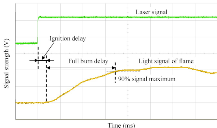
FIGURE 6 Oscilloscope traces of laser and the ignited flame during a laser ignition process, defining the ignition delay and full burn delay.
