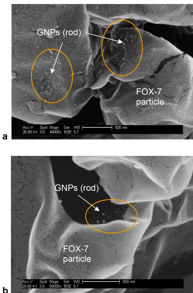
FIGURE 11 SEM images of sensitized FOX-7 with a) Citrate capped GNPs and b) CTAB capped GNPs.
