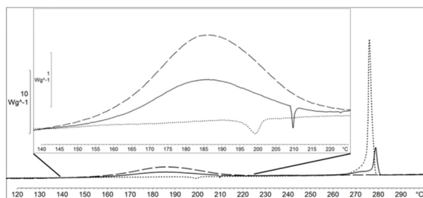
Figure 9 Thermograms of HMX (dotted line), \beta NCPD1 (dashed line) and the mixture (solid line) at 2 °C min -1 .
