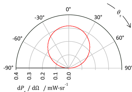
Fig. 6. Level of light reflected from a perfectly Lambertian surface P_r per unit solid angle \Omega (as dP_r/d\Omega ) as a function of collection angle \theta , for an incident beam of power 1 mW.
