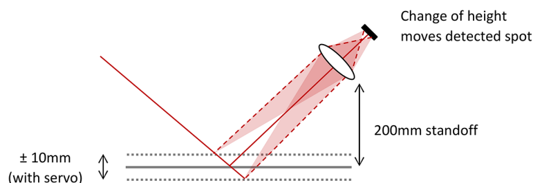
Fig. 7. If the surface height changes, a parallax effect causes movement of the detected spot on the photodetector. To detect all laser beams equally, the photodetector must be larger than the extent of the movement imaged at its location.
