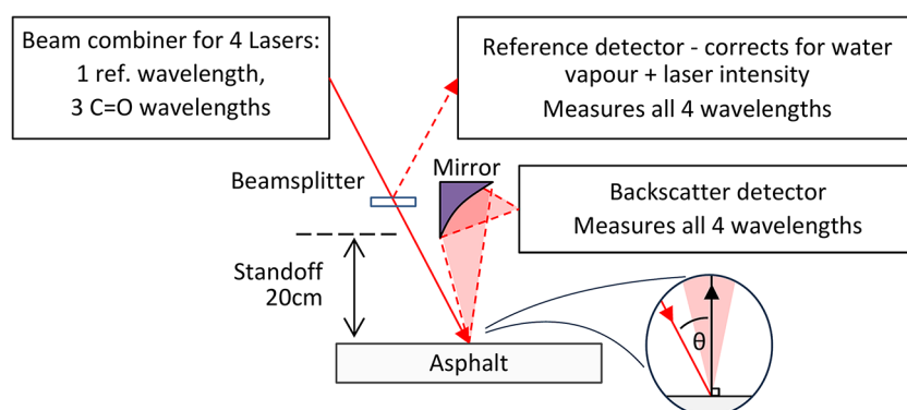
Fig. 3. Measurement principle for standoff measurement of diffuse reflection at 4 wavelengths, 3 across the C=O band and one at a reference wavelength. Two detectors are used, one to measure the backscattered light at each wavelength, and a pathlength-matched reference detector to correct for laser output variation and residual water vapour absorption. Inset shows the angle of incidence, \theta .
