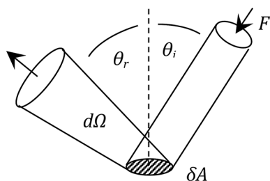
Fig. 5. Geometric definitions used to describe diffuse reflection.
