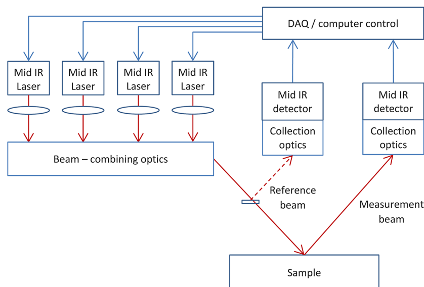
Fig. 8. Schematic diagram of concept for instrument for laser-based spectral analysis of roads. (DAQ digital acquisition system). Note that reference and measurement beams should be pathlength-matched.
