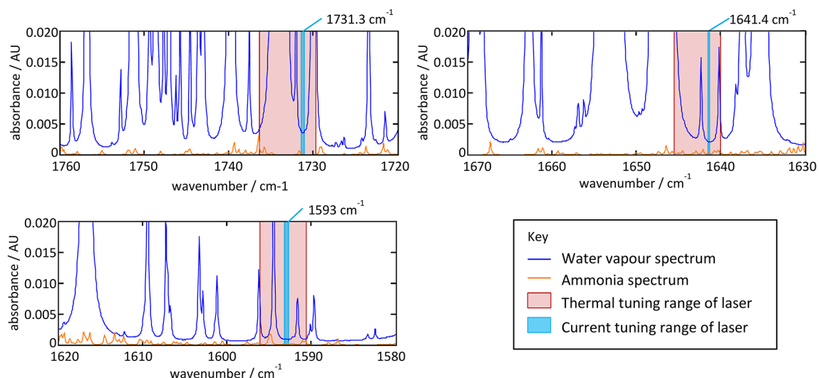
Fig. 4. Tuning ranges for the three lasers chosen to span the carbonyl region, overlaid onto spectra for water vapour (6%vol) and ammonia (900 ppm) for a pathlength difference of 2.2 cm. The thermal and current tuning ranges show the full range of wavelengths accessible to each laser, and range corresponding to rapid injection current modulation, respectively. Y-axis absorbance figures translate directly into uncertainty in the measurement of asphalt.
