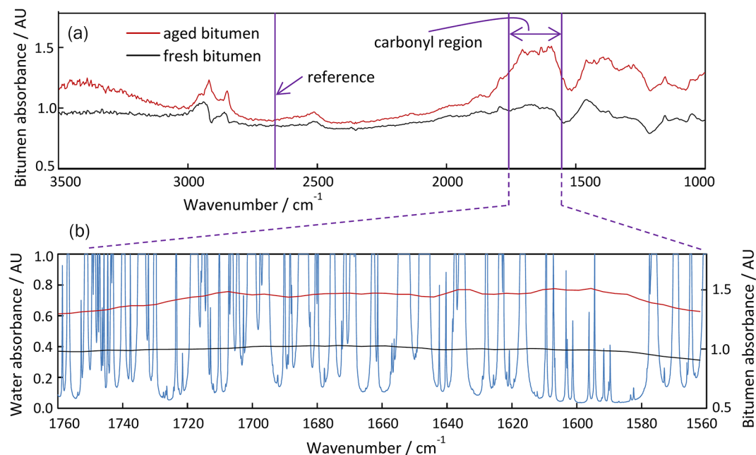
Fig. 2. (a) Diffuse reflectance spectra measurement with a hand-held FTIR spectrometer, for aged and fresh bitumen within asphalt samples 25 . (b) Section of bitumen spectra overlaid on absorption spectrum for atmospheric water vapour, calculated from the PNNL database for an optical pathlength of 1m and 6.6%vol (worst-case abundance at 90% RH and 40 °C).
