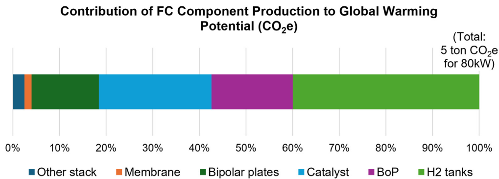
Fig. 45. Global warming potential (CO 2 e) of the production of a FC system and gaseous H 2 tank with 80 kW net power output and contribution of components in automotive applications. Source: Adapted from [130].
