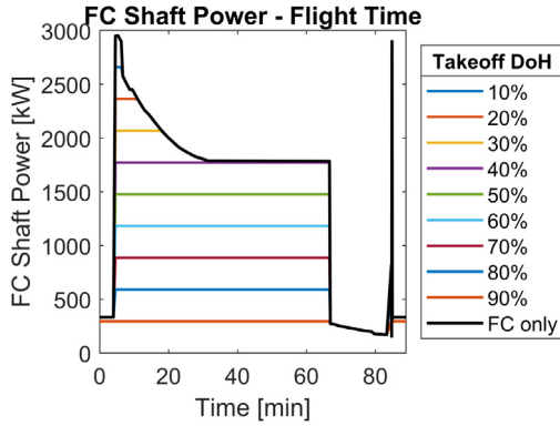
Fig. A.51. Electric power provided by the FC in a hybrid FC+battery system for different take-off DoH at NPPC = 3 kW/kW.
