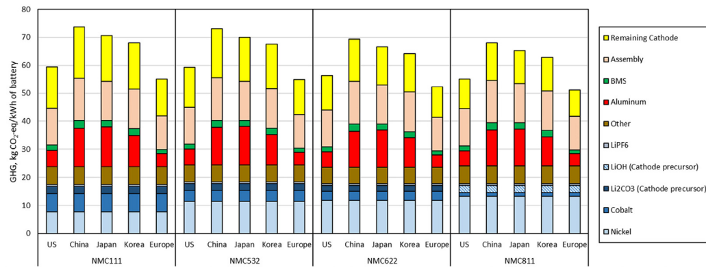
Fig. 44. Battery production CO 2 e for different regions and cells. Source: Reprinted from [127] under CC BY-NC-ND 4.0 licence.
