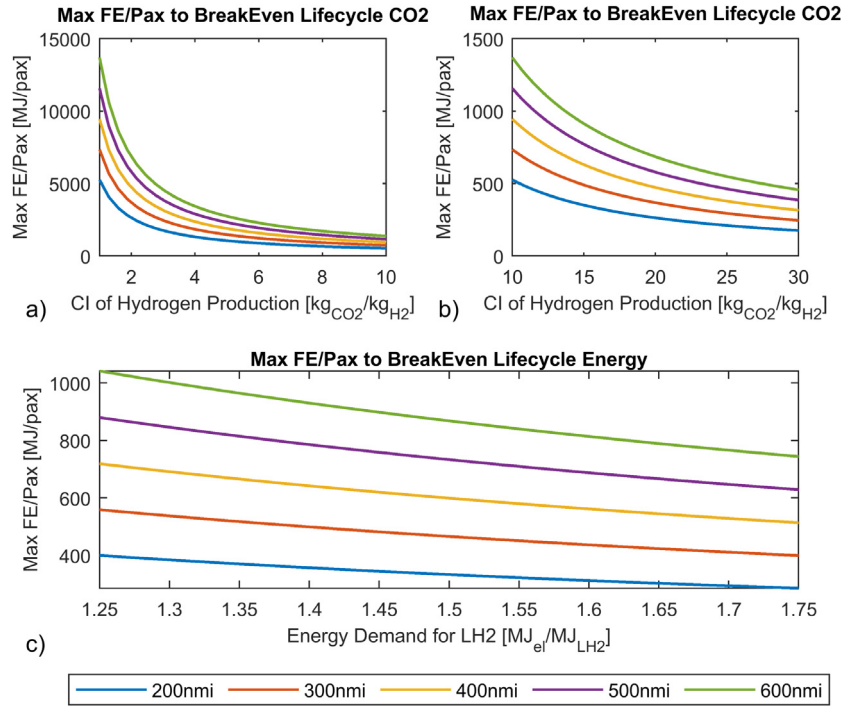
Fig. 24. Flight energy per pax target to breakeven lifecycle CO 2 and lifecycle energy of the conventional regional aircraft.
