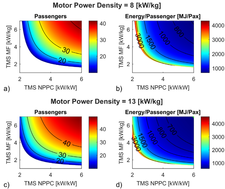
Fig. 6. Trade-off in TMS NPPC and TMS mass factor along with benefits from motor technology upscaling for FC aircraft. The green line represents the energy/pax of today's 50-pax regional aircraft.
