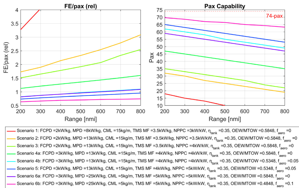
Fig. 46. Technology scenarios for FC aircraft for 200–800 nmi.
