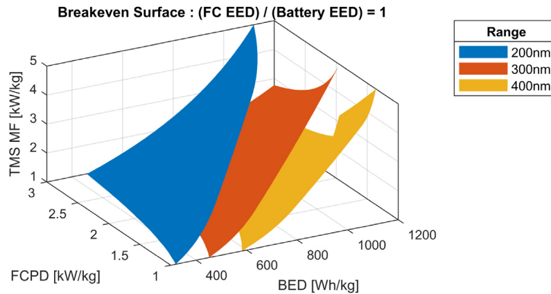
Fig. 15. Breakeven surface between FC and battery system for three ranges.
