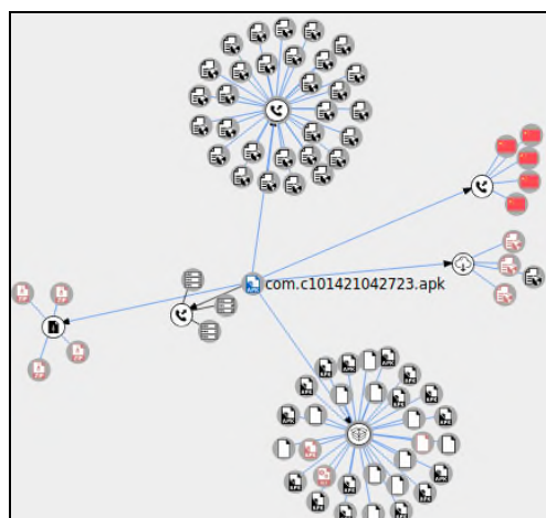
Fig. 9. Malware Activity connectivity
