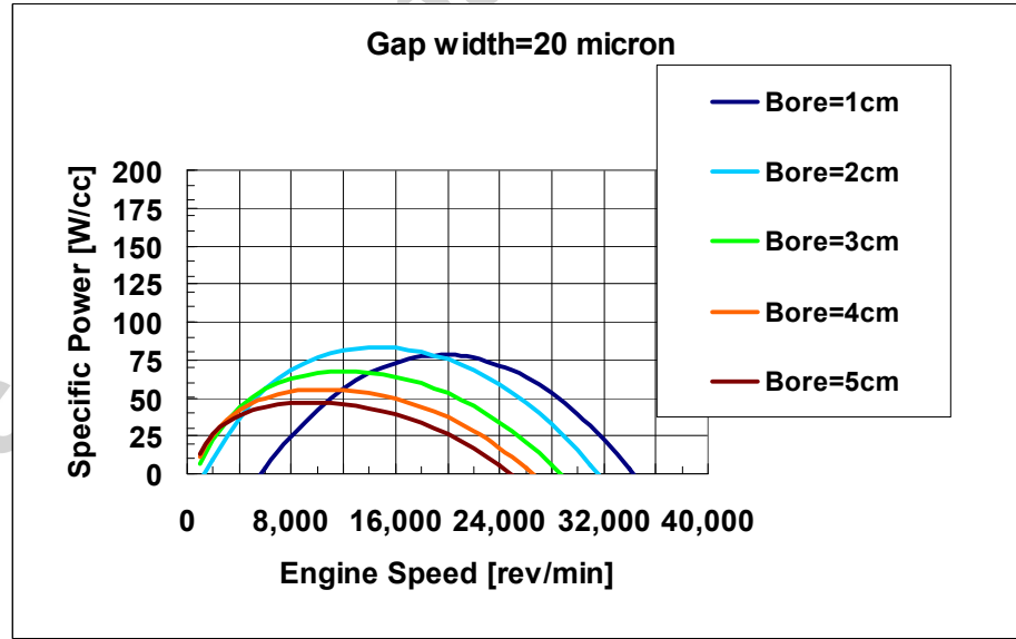
Figure 4b: The corresponding specific brake engine power.
