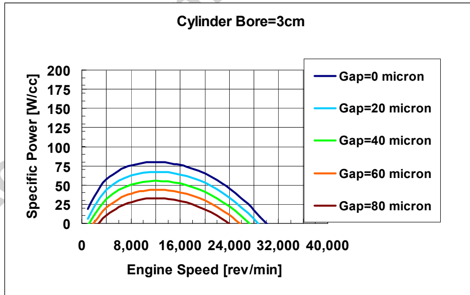
Figure 3b: The corresponding specific brake engine power.
