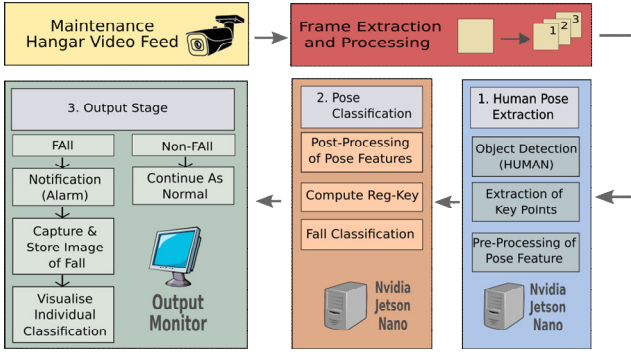
Fig. 1. Proposed Fall Detection System Architecture
