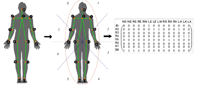
Fig. 2. Reg-Key Process Visualized.
