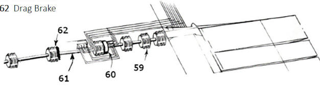
(a) Sketch of the XB-70 actuator system layout
