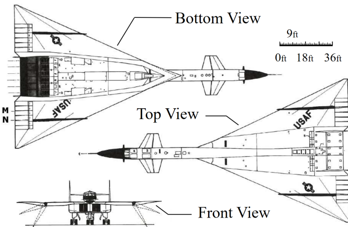
(a) XB-70 Geometric Drawings
