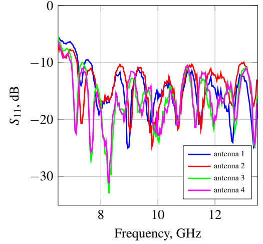
Figure 8. Measured S_{11} reflection coefficient for individual antennas in the polarimetry array (see Fig. 7 inset to locate individual antennas).
