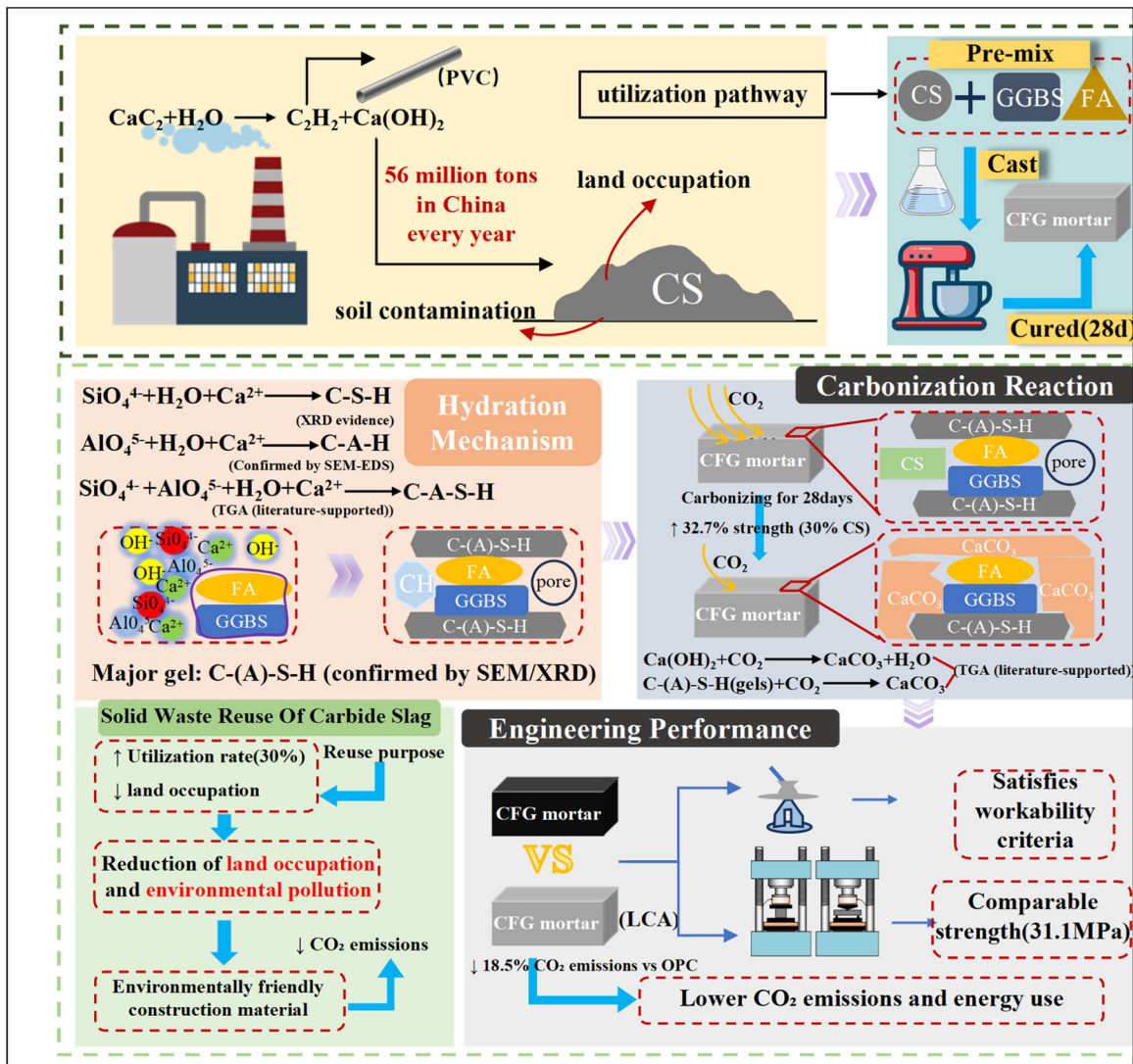
Fig. 11. Performance improvement and environmental friendliness of CFG.
