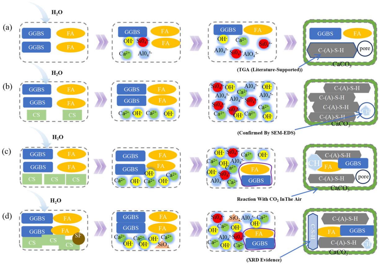
Fig. 7. Speculated hydration mechanism: (a) CFG without CS; (b) CFG with a small amount of CS; (c) CFG with excessive CS; (d) CFG with SF.
