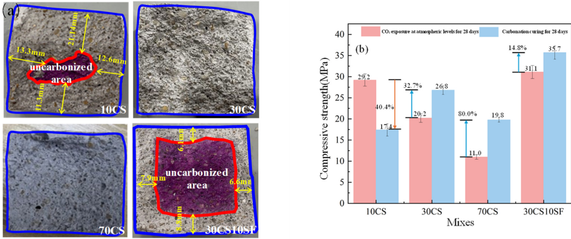
Fig. 8. Performance changes of CFG system after carbonization: (a) carbonization depth of different groups; (b) effect of carbonization on mechanical properties.
