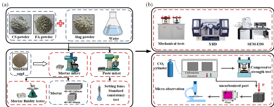
Fig. 2. Preparation and test flow chart of CFG cementitious material: (a) preparation of specimens and working performance tests; (b) mechanical property tests, microanalysis, and carbonization tests.
