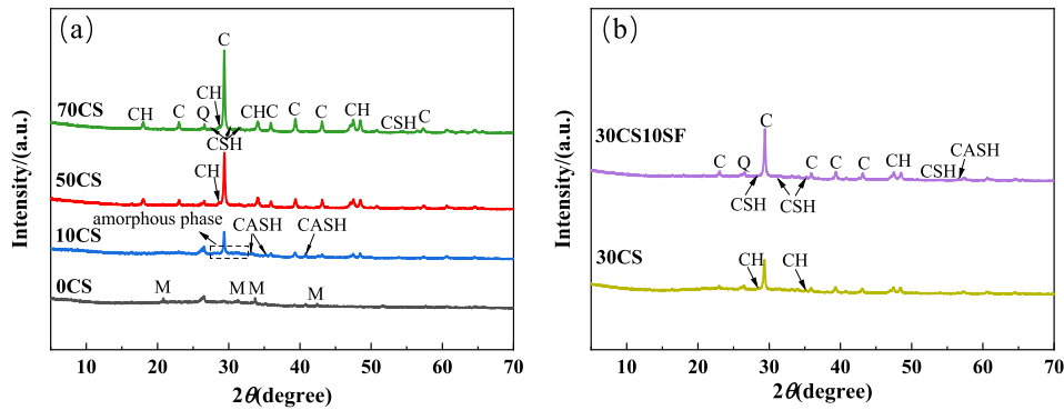
Fig. 5. XRD results of the CFG at 28d: (a) effect of different CS dosages; (b) effect of SF dosage, Note: M: mullite; Q: quartz; C: calcite; CASH: calcium aluminate silicate hydrates; CSH: calcium silicate hydrates; CH: calcium hydroxide.
