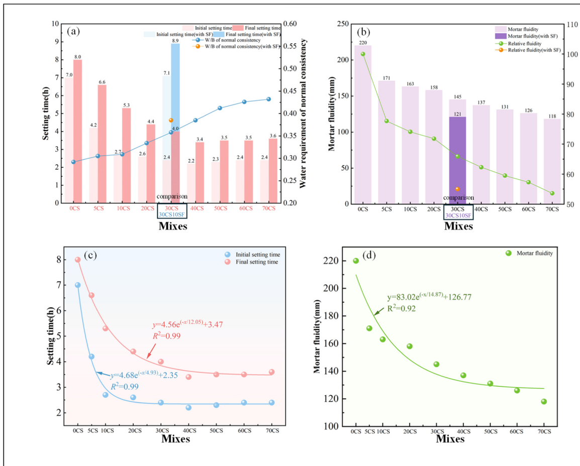
Fig. 3. The workability of CFG: (a) setting time and water requirement of standard consistency; (b) mortar fluidity; (c) fitting relationship of setting time; (d) fitting relationship of mortar fluidity.
