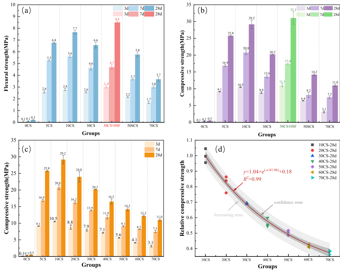
Fig. 4. Mechanical properties of CFG under different curing ages and CS dosages: (a) flexural strength of characteristic mixes; (b) compressive strength of characteristic mixes; (c) compressive strength of all mixes; (d) fitting relationship between compressive strength and CS dosage.
