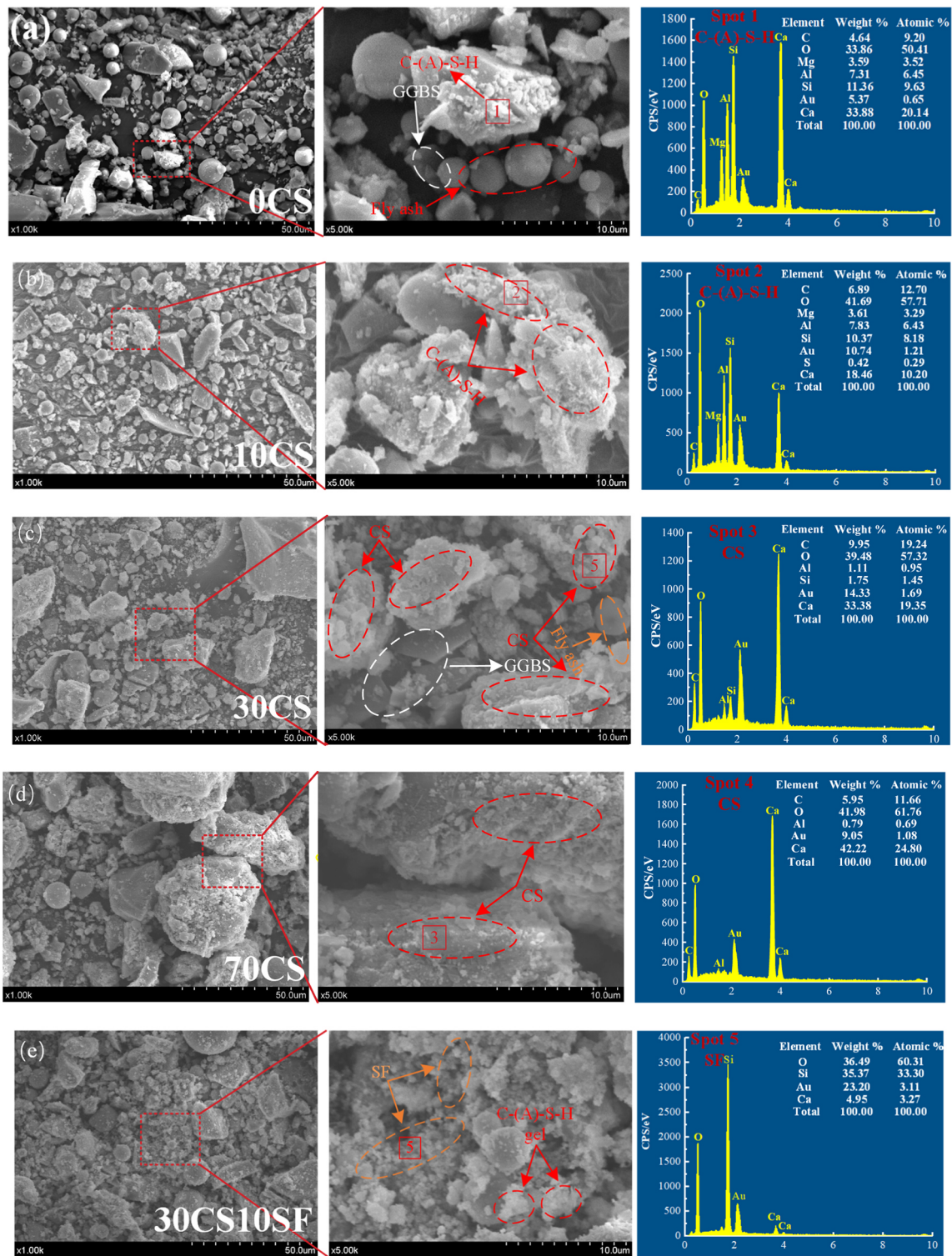
Fig. 6. The SEM and EDS results of the CFG system with different parameters at 28d: (a) 0CS; (b) 10CS; (c) 30CS; (d) 70CS; (e) 30CS10SF.
