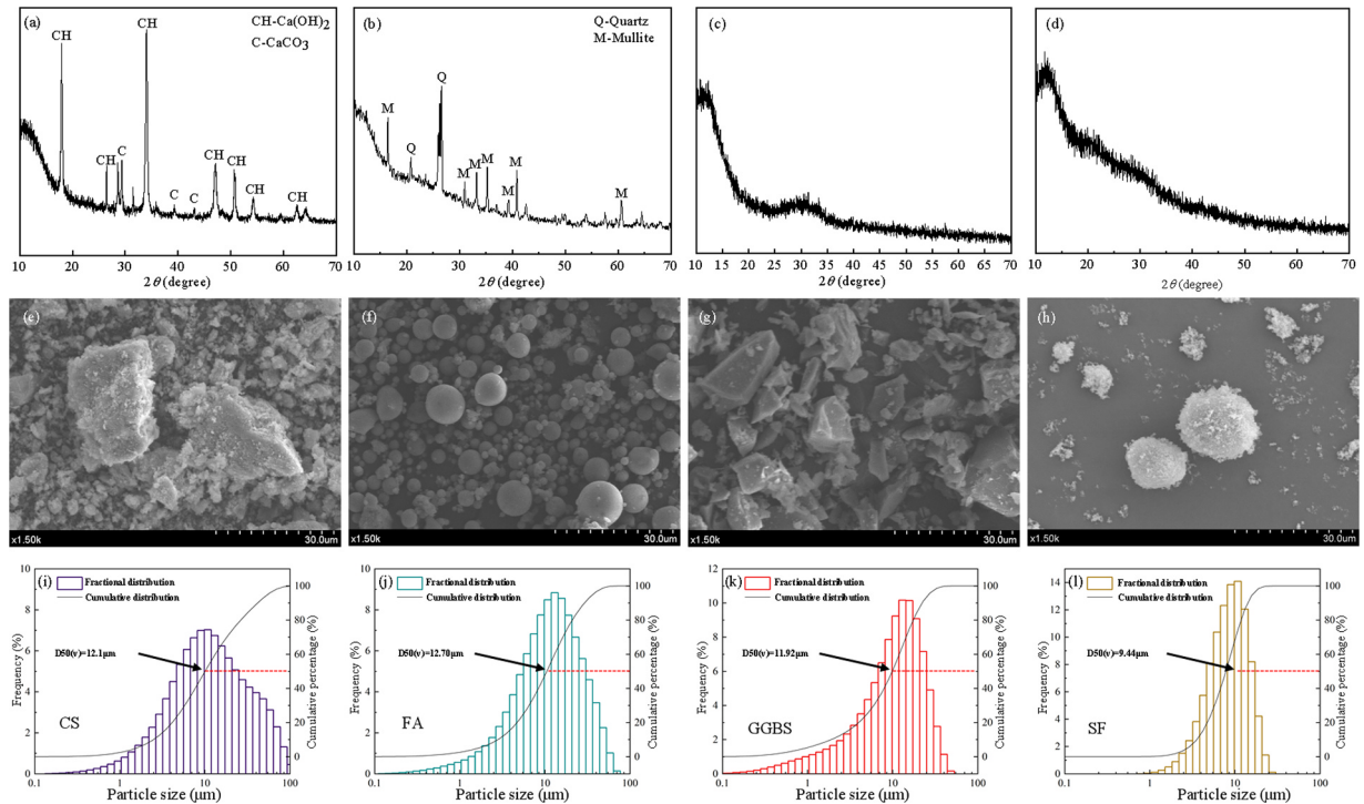
Fig. 1. XRD, SEM and PSD analysis of raw materials: (a) XRD of CS; (b) XRD of FA; (c) XRD of GGBS; (d) XRD of SF; (e) SEM of CS; (f) SEM of FA; (g) SEM of GGBS; (h) SEM of SF; (i) PSD of CS; (j) PSD of FA; (k) PSD of GGBS; (l) PSD of SF.
