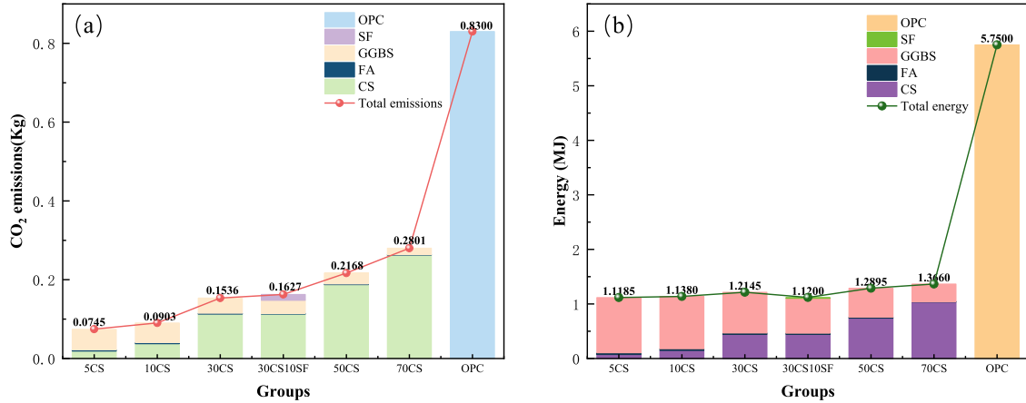
Fig. 10. CO 2 emissions and energy consumption of different pastes: (a) CO 2 emissions of different pastes; (b) energy consumption of different pastes.
