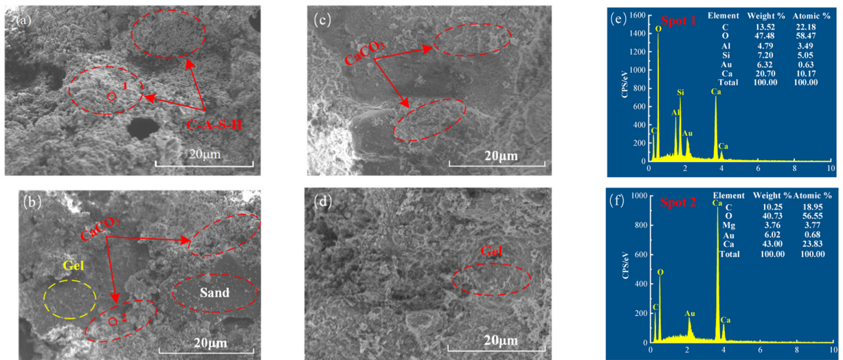
Fig. 9. SEM-EDS characterization of samples after 28 days of carbonization: (a) 10CS; (b) 30CS; (c) 70CS; (d) 30CS10SF; (e) EDS of spot 1; (f) EDS of spot 2.
