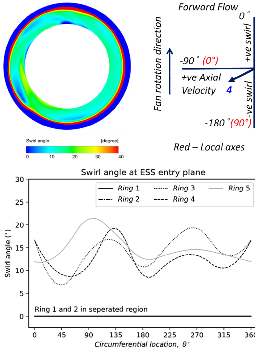
FIGURE 10: SWIRL ANGLE DISTRIBUTION INTO CORE ENGINE
