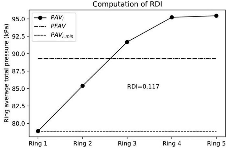
FIGURE 9: COMPUTATION OF RADIAL TOTAL PRESSURE DISTORTION INDEX
