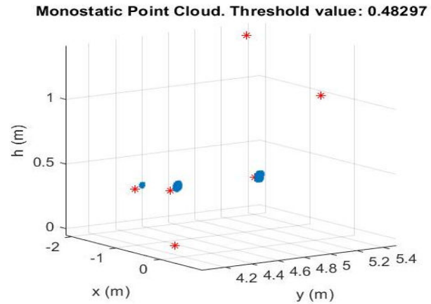
Figure 12: SAR Point Cloud rendering from data collected in the laboratory. Blue point clouds indicate the algorithm detections, and scatterer ground truth positions are marked by red asterisks.
