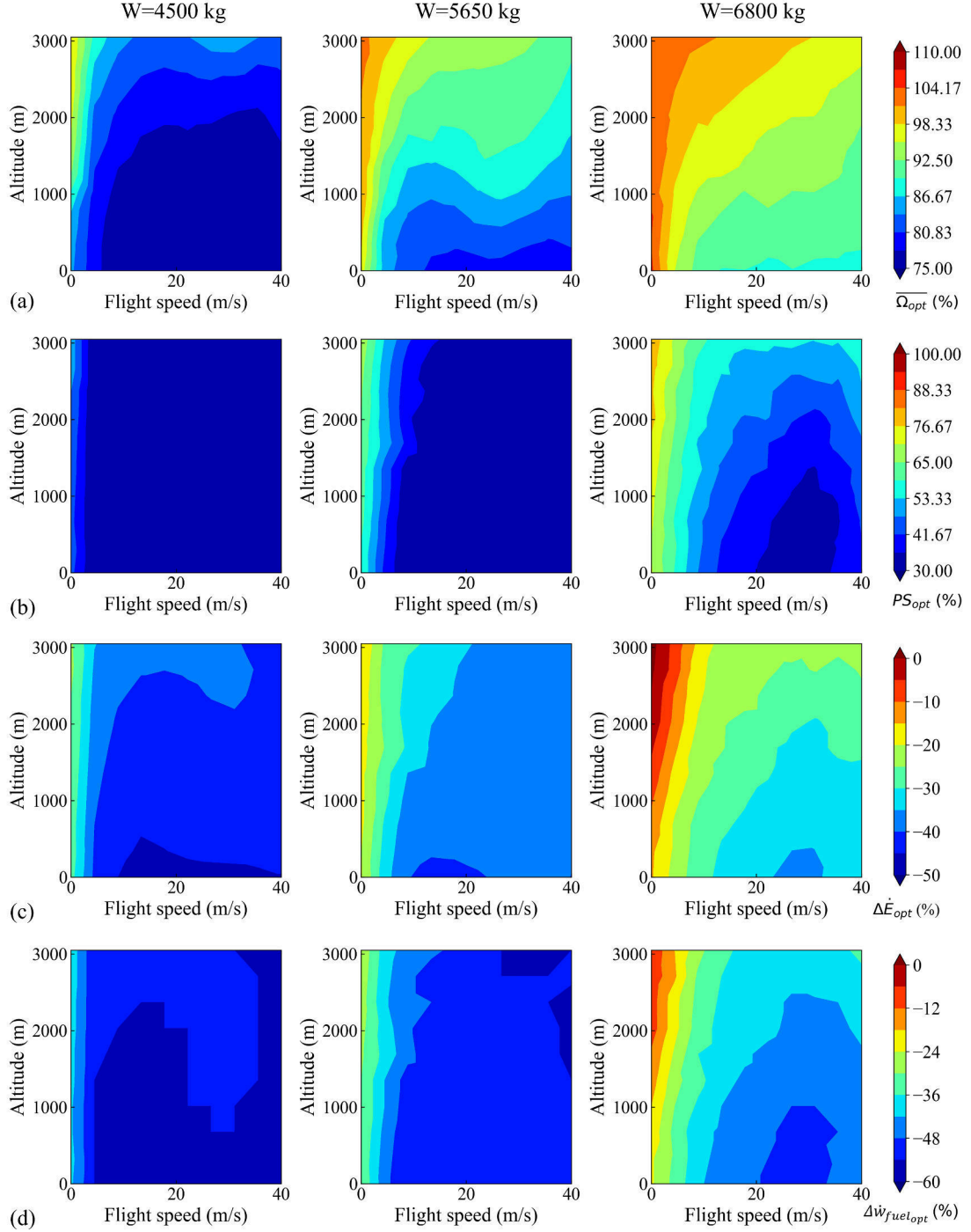
Figure 9: Optimized control schedule for variable \Omega and PS at \phi_{tilt}=90^\circ as function of gross weight W , altitude h and rotorcraft speed V : (a) optimum rotor speed variation \overline{\Omega}_{opt} (%), (b) optimum power split PS_{opt} (%), (c) resultant energy rate relative to the nominal configuration \Delta \dot{E}_{opt} (%) and (d) resultant fuel flow relative to nominal configuration \Delta \dot{w}_{fuel_{opt}} (%)
