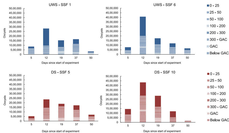
Fig. 4. Cryptosporidium oocysts retained in each layer for all cores for underwater and dry skimmed duplicate slow sand filters.
