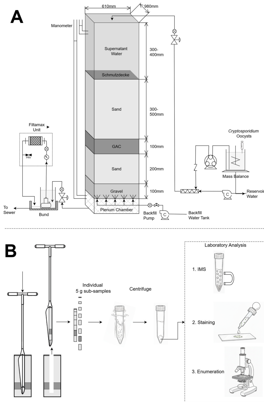
Fig. 1. (A) Diagram of the pilot-scale slow sand filtration system in its setup for the dosing experiment, (B) Flowchart of the sampling and sectioning of the SSF core, the sandwashing step to detach the particulate matter from the sand grains, followed by the IMS isolation, staining and enumeration of oocysts.
