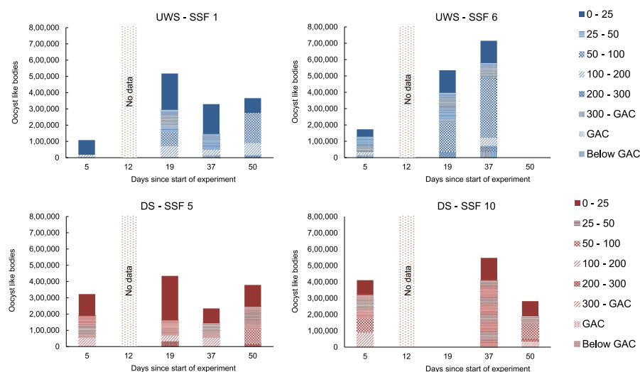
Fig. 5. Oocysts-like bodies (OLB) retained in each layer for all cores for underwater and dry skimmed duplicate slow sand filters.
