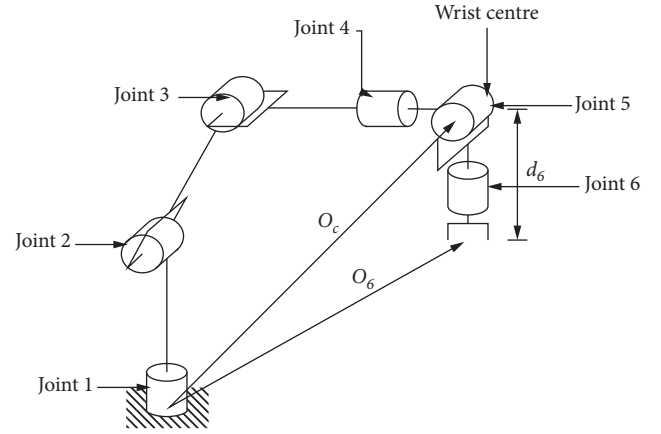
FIGURE 7: Kinematics decoupling (Spong, Hutchinson, and Vidyasagar, 2006).
