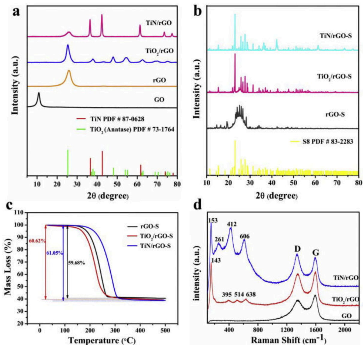
Fig. 4. (a) XRD pattern of GO, rGO, \text{TiO}_2/\text{rGO} and \text{TiN}/\text{rGO} , green and red drop lines correspond to anatase \text{TiO}_2 (PDF # 73–1764) and TiN (PDF # 87–0628); (b) XRD pattern of \text{rGO-S} , \text{TiO}_2/\text{rGO-S} and \text{TiN}/\text{rGO-S} , yellow drop lines correspond to sulfur (PDF # 83–2283); (c) TG curves of \text{rGO-S} , \text{TiO}_2/\text{rGO-S} and \text{TiN}/\text{rGO-S} ; (d) Raman spectra of GO, \text{TiO}_2/\text{rGO} and \text{TiN}/\text{rGO} .
