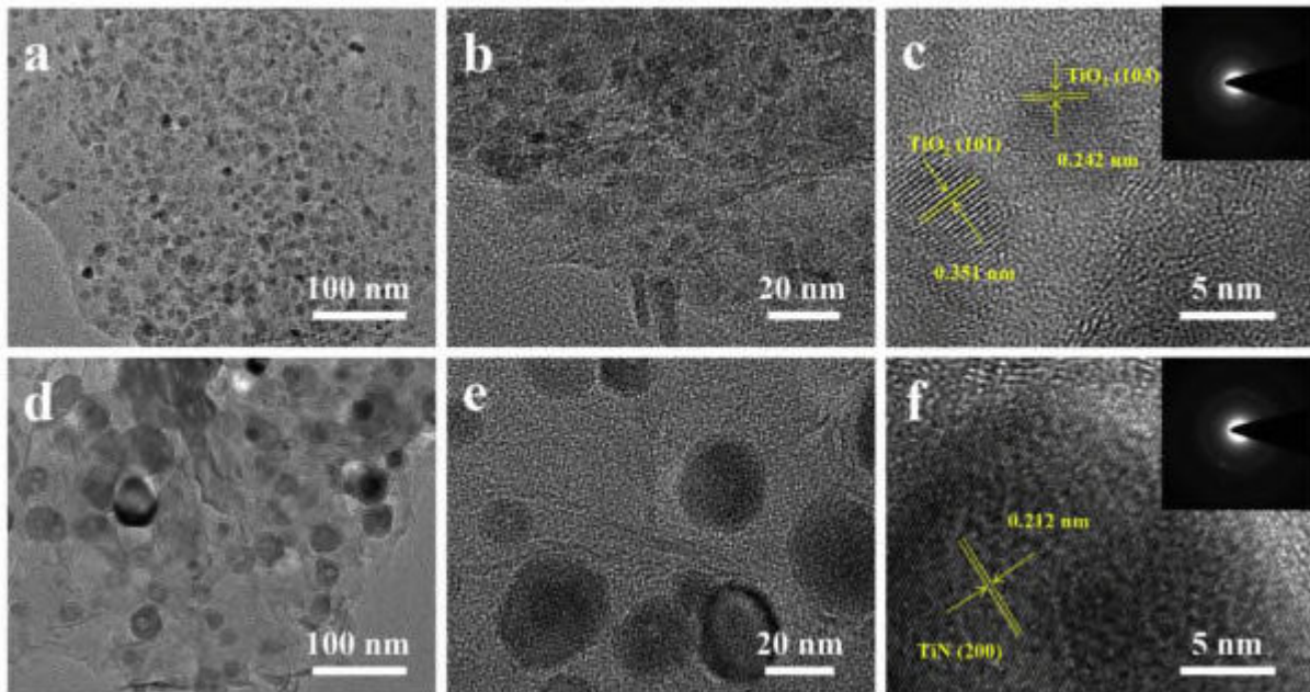
Fig. 3. (a–c) low magnification and high resolution TEM of the anatase TiO 2 /rGO; (d–f) low magnification and high resolution TEM of the TiN/rGO.
