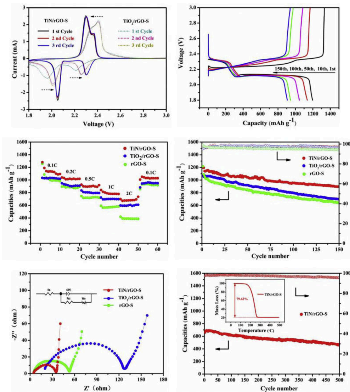
Fig. 5. Electrochemical performance. (a) CV profiles of \text{TiO}_2/\text{rGO-S} and \text{TiN/rGO-S} cathodes; (b) charge-discharge profiles of \text{TiN/rGO-S} cathode over different cycles at a current rate of 0.1C; (c) rate capacity, (d) cycling performance at 0.1C and (e) EIS spectra of \text{rGO-S} , \text{TiO}_2/\text{rGO-S} and \text{TiN/rGO-S} cathodes before cycling; (f) cycling performance of \text{TiN/rGO-S} cathode (with the sulfur content of 79.62% wt.) at a current rate of 1C.
