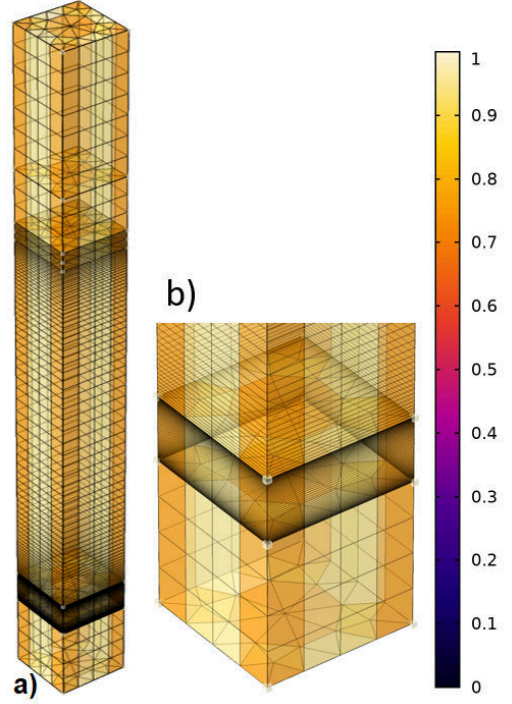
Figure 2: a. The mesh quality for skewness (overall geometry), and b. Mesh quality for Mo(S,Se) 2 layer
