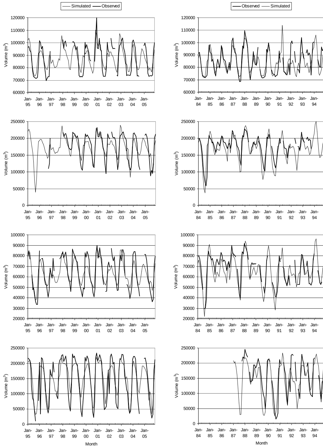
Figure 7 Simulated and observed lake volumes in the (from top) Upper Eastern Arm; Lower Eastern Arm; Central Arm; Central Lake-Western Arm during the (left) calibration and (right) validation periods.
