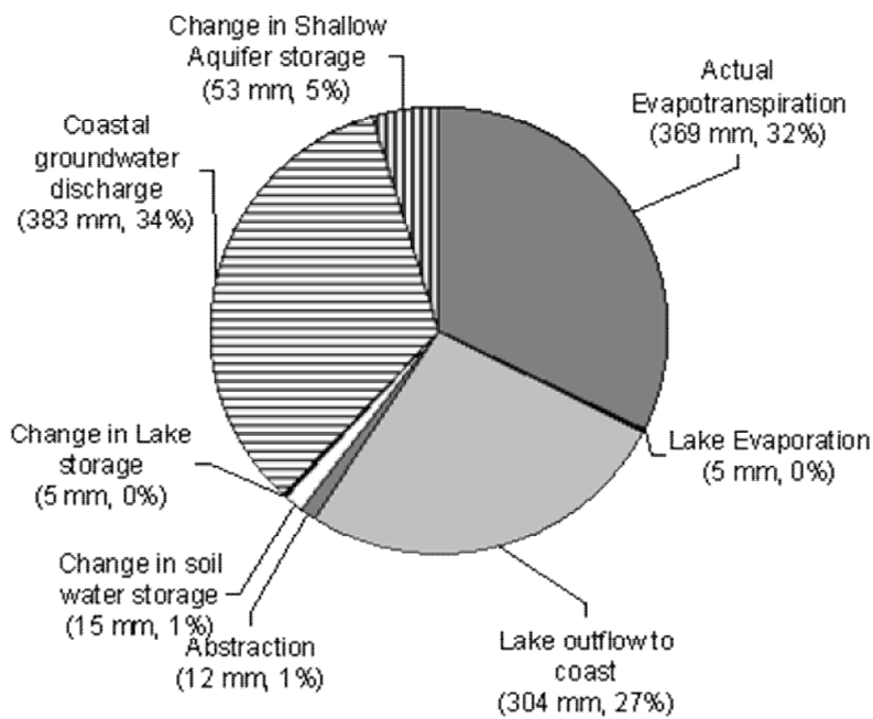
Figure 9 Water budget for the Bosherton system (years 1984-1994).
