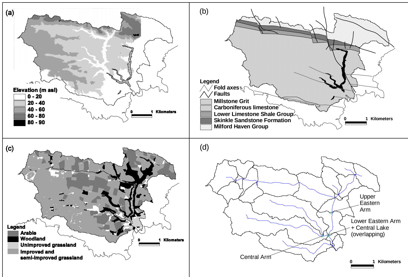
Figure 2 Bosherton catchment - (a) elevation, (b) bedrock geology, faults and fold axes and generalised cross section; (c) land use; (d) SWAT representation of the catchment and waterbodies [Geological Map Data © NERC 2009; Elevation data © Ordnance Survey 2009]
