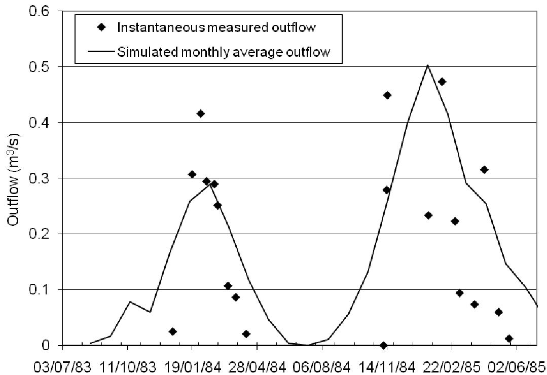
Figure 8 Modelled monthly average and instantaneous measured lake outflows to the sea during the validation period
