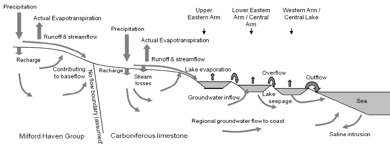
Figure 4 Conceptual model of the Bosherton Lakes system
