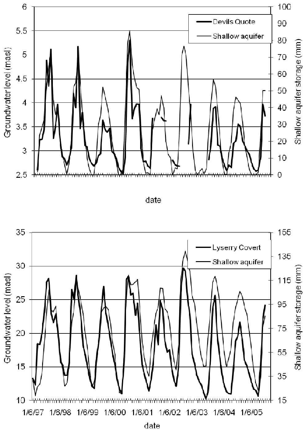
Figure 6 Comparison of observed groundwater levels and simulated SWAT shallow aquifer storage within the catchment during the calibration period at Devils Quote and Lysserry Covert boreholes.
