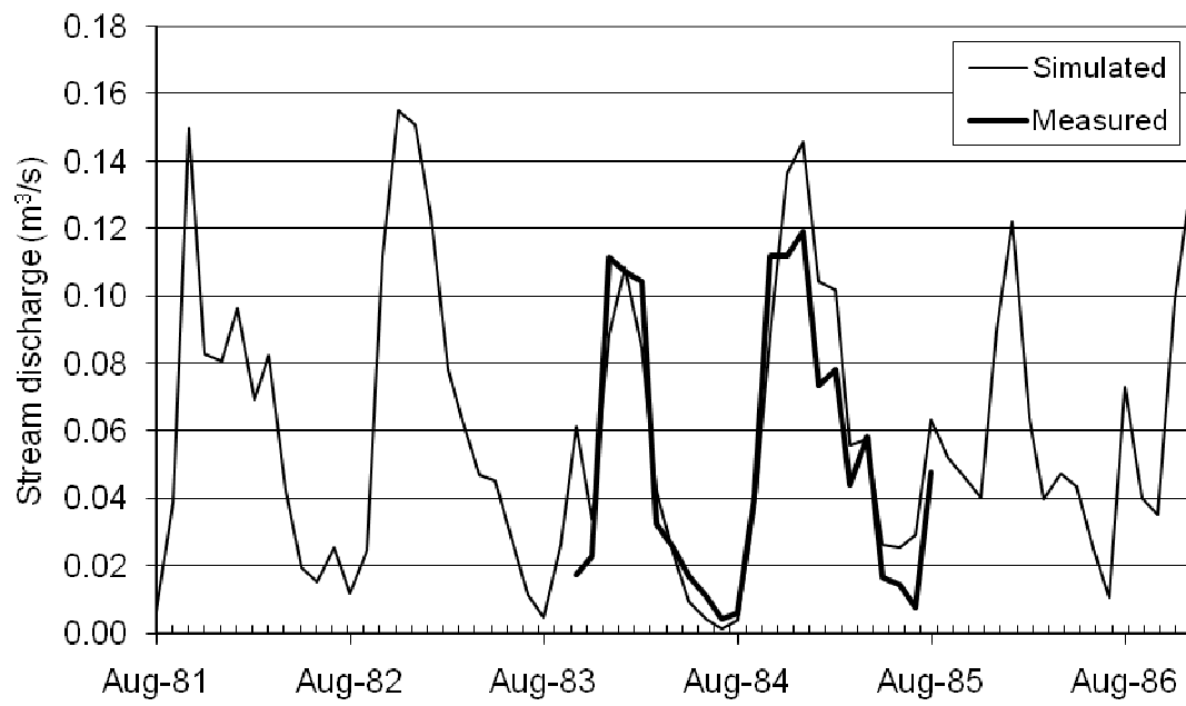
Figure 5 Measured and simulated average monthly flows in Stackpole Stream during the calibration period
