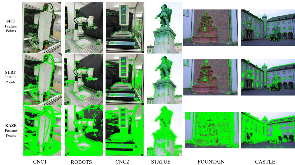
Figure 12. Demonstration of the three kinds of feature descriptors used on Dataset 1 and Dataset 2.
