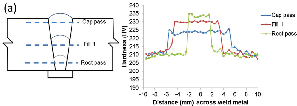
Fig. 16. As-welded (a) hardness scan position (b) Hardness profile across the multi-pass welds.
