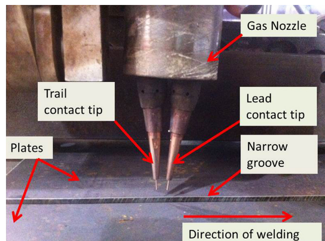
Fig. 2. Typical tandem GMAW torch.
