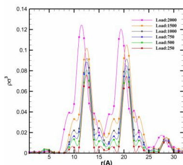
Adsorption of Argon for (10 \times 10) SWCNT
