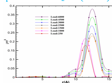
Adsorption of Ar- \text{CO}_2 for (16 \times 16) SWCNT
