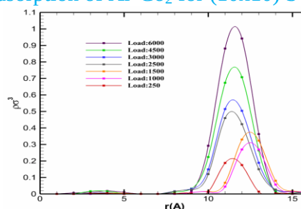
Adsorption of Ar- \text{CO}_2 for (10 \times 10) SWCNT
