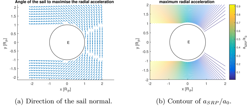
Figure 2: Maximisation of radial acceleration, for a single-sided coating sail around Earth subject to SRP.
