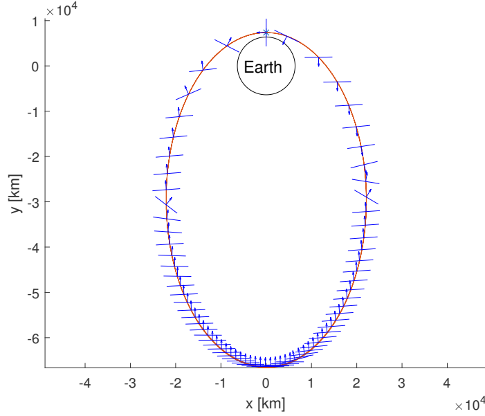
Figure 8: Trajectory around the Earth with orientation of the sail on T2 ( \omega_0 = 90 \text{ deg} ) considering SRP+PRP.
