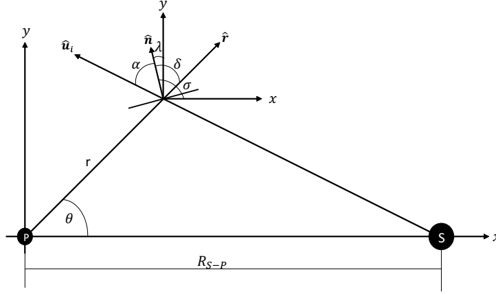
Figure 1: Reference frame for a sail orbiting around a planet.
