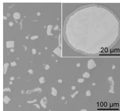
Figure 2. Microstructure of the Ti@Al 3 Ti core-shell particle-reinforced Al matrix composite (annealing of the spark plasma sintered and hot-rolled material at 600 °C for 2 h). Inset: a core-shell particle. Reprinted from [9], Copyright (2020), with permission from Elsevier.
