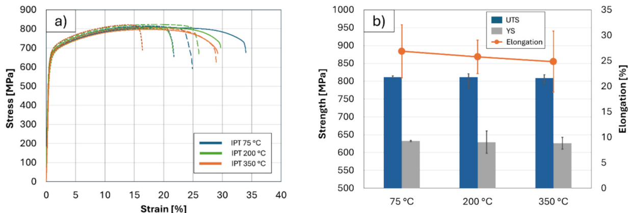
Fig. 13. a) Room temperature tensile results of SDSS CW-GMA a) Stress-strain curve, b) Average UTS, YS, and elongation results at different interpass temperatures.
