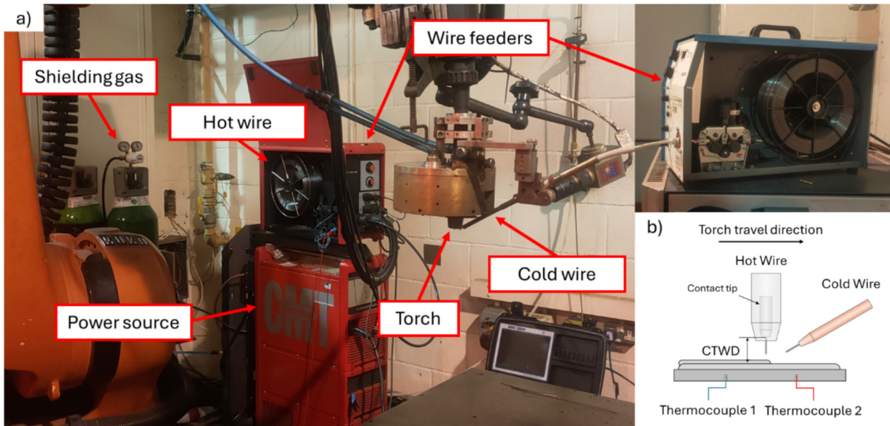
Fig. 1. a) CW-GMA Experimental setup. b) Illustration of CW-GMA wires and thermocouple position.
