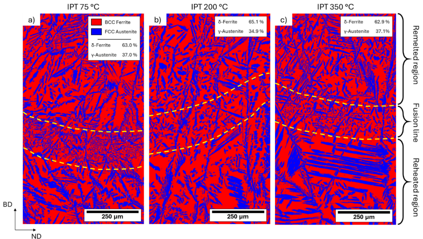
Fig. 6. Phase maps of higher magnification EBSD under different interpass temperatures: a) 75 °C; b) 200 °C; c) 350 °C.
