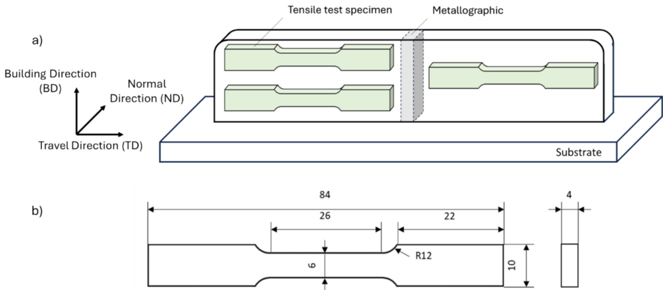
Fig. 2. a) Illustration of the CW-GMA walls with the location of specimens used for uniaxial tensile. b) Tensile specimen dimensions.
