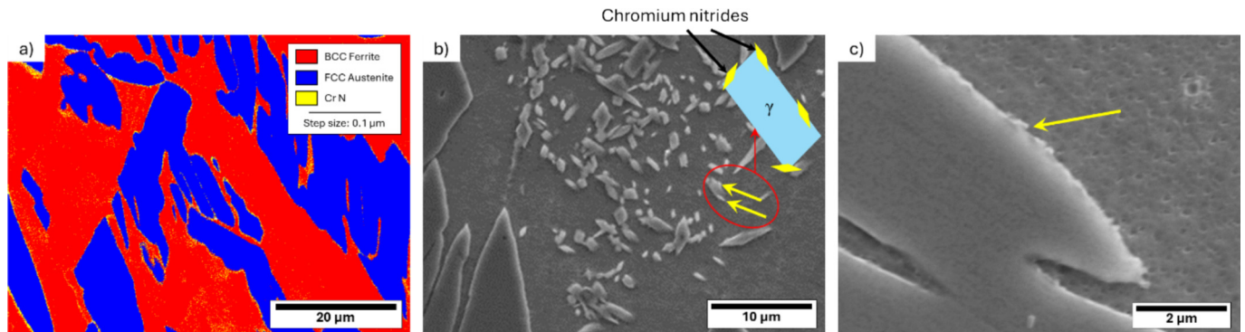
Fig. 10. Identification of CrN using EBSD analysis a), SEM image of fine secondary austenite region b) and high magnification austenite grain boundary c). Chromium nitrides indicated by yellow arrows. (For interpretation of the references to colour in this figure legend, the reader is referred to the web version of this article.)
