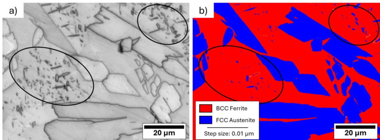
Fig. 9. Secondary austenite identification by EBSD a) Band contrast b) IPF map.
