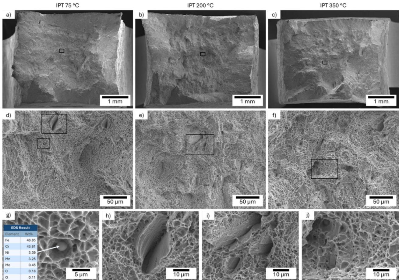
Fig. 14. Fracture morphology of tensile specimens at difference magnifications (a, d, g, h) IPT of 75 °C (b, e, i) IPT of 200 °C (c, f, j) IPT of 350 °C.
