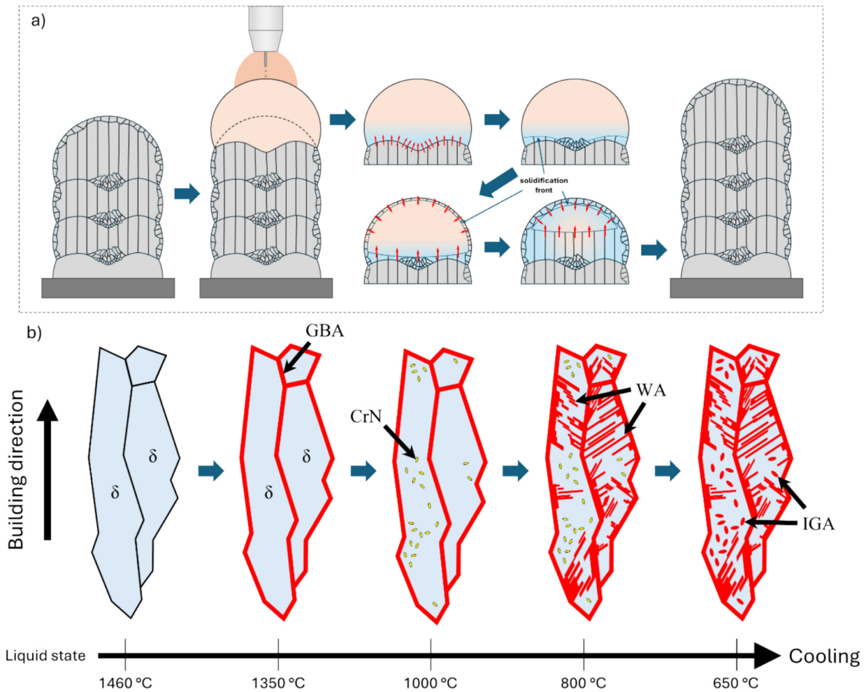
Fig. 11. a) Schematic representation of ferrite grain growth during the CW-GMA process for SDSS, b) Schematic representation of microstructure evolution during cooling in the CW-GMA process for SDSS.
