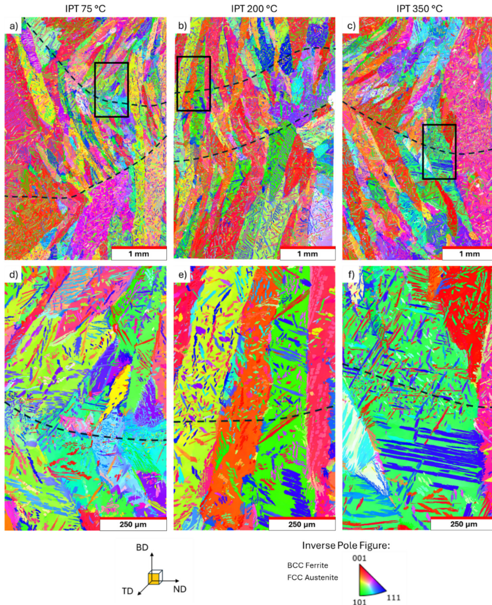
Fig. 5. Inverse pole figures from EBSD analysis of SDSS CW-GMA walls under different interpass temperatures. Low magnification: a) 75 ^{\circ}\text{C} , b) 200 ^{\circ}\text{C} , c) 350 ^{\circ}\text{C} . High magnification: d) 75 ^{\circ}\text{C} , e) 200 ^{\circ}\text{C} , f) 350 ^{\circ}\text{C} .
