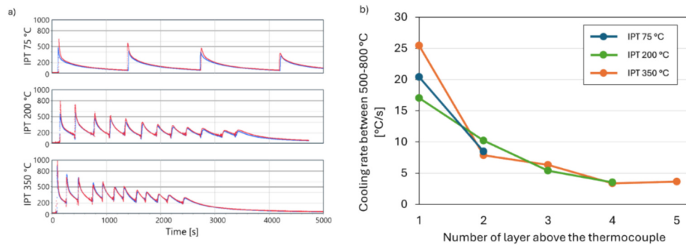
Fig. 3. a) Thermal cycles from the thermocouples; b) Average cooling rates from 800 °C to 500 °C of each pass under different interpass temperature conditions.
