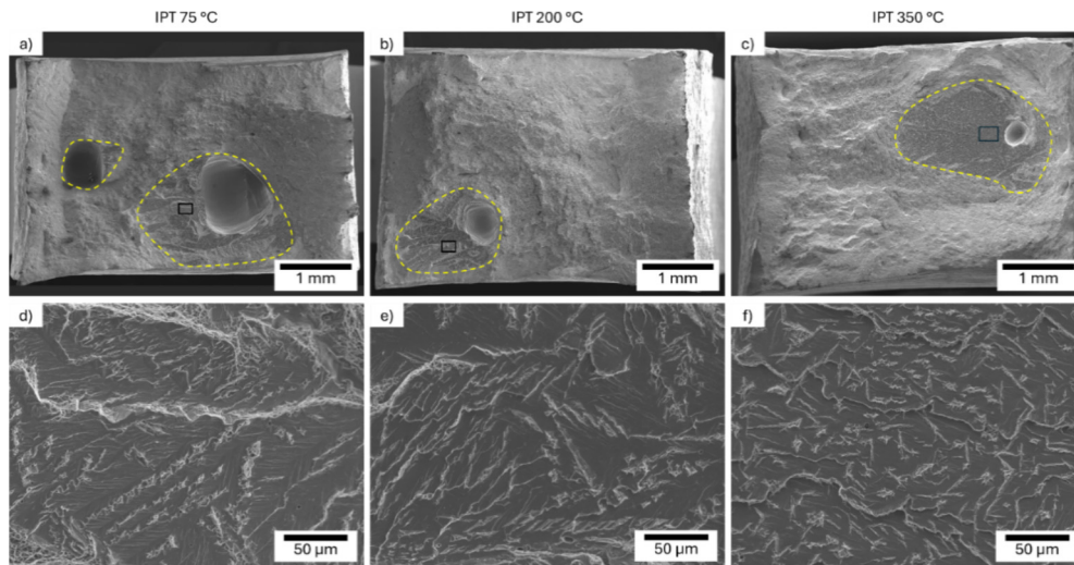
Fig. 15. Fracture morphology of tensile specimens with low elongation at difference magnifications (a, d) IPT of 75 °C (b, e) IPT of 200 °C (c, f) IPT of 350 °C.
