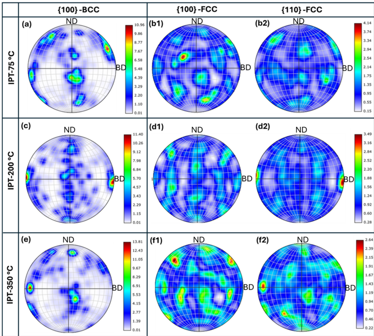
Fig. 8. Phase pole figures for {100} BCC ferrite (a, c, e), {100} FCC austenite (b1, d1, f1), and {110} FCC austenite (b2, d2, f2), oriented along the normal direction (ND) and building direction (BD) for SDSS processed via CW-GMA under interpass temperatures.
