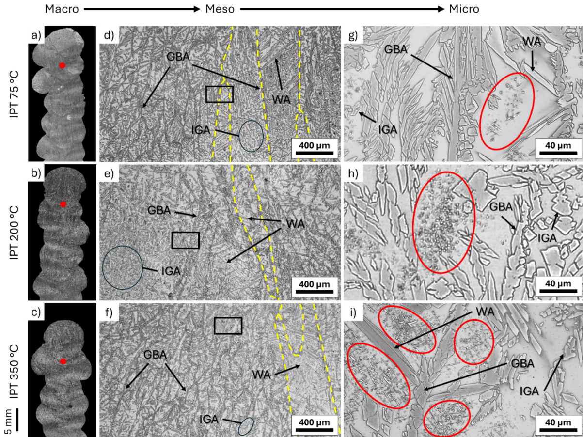
Fig. 4. Cross-section macrographs and microstructure at different magnifications of SDSS CW-GMA walls under different interpass temperatures: (a, d, g) 75 °C; (b, e, h) 200 °C; (c, f, i) 350 °C.
