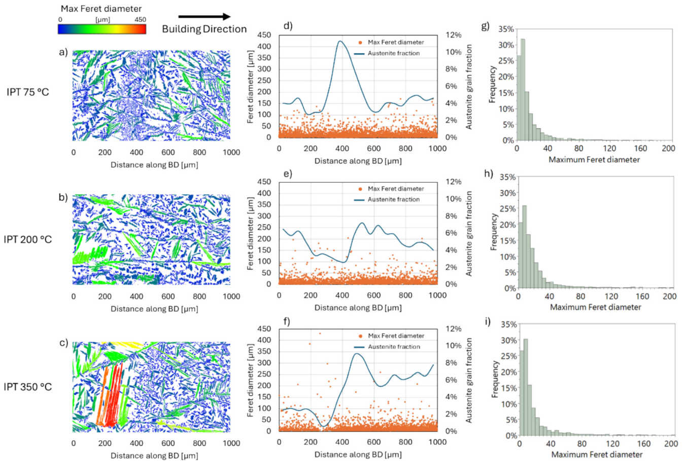
Fig. 7. Austenite phase size analysis at layer transition. a–c) EBSD Maximum Feret diameter d–f) Austenite phase size across the fusion line g–i) Maximum Feret distribution.
