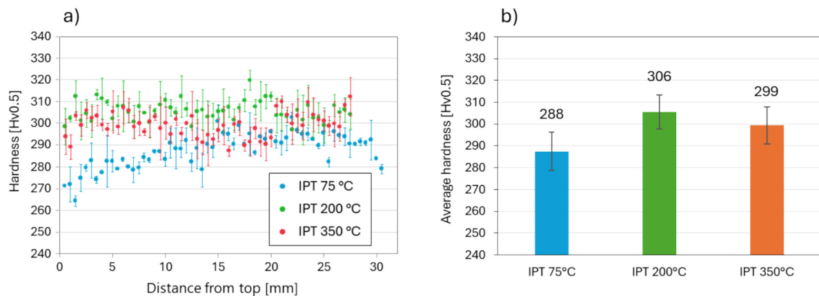
Fig. 12. a) Micro-hardness profile of SDSS CW-GMA process walls. b) average hardness with different interpass temperatures.
