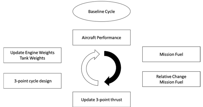
Figure 6: 3-point thrust requirements iteration process
