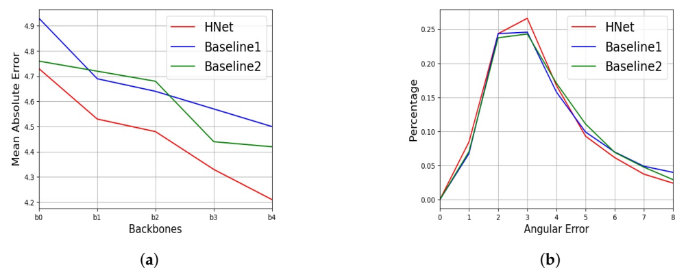
Figure 7. The mean absolute error and percentage of angular errors on the AFLW2000 dataset: (a) the mean absolute error when different versions of EfficientNet (b0–b4) were used as the feature extractor; (b) the percentage of angular errors using EfficientNet-b4.
