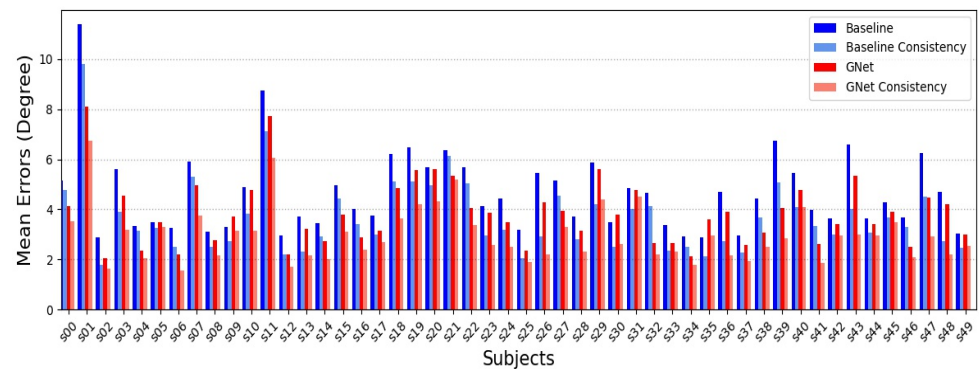
Figure 8. A comparison between the results from the baseline model and the proposed GNet model, both with and without the gaze consistency principle, for different subjects from the UT-Multiview dataset.
