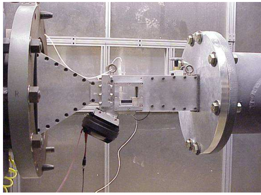
(a) Wind tunnel with recessed cavity
