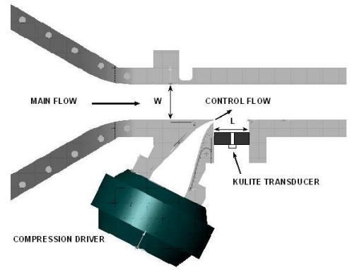
(b) Geometry of the test section
