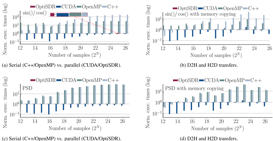
Fig. 6 Runtime performance for the same dataset against different serial and parallel programming models
