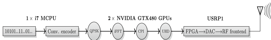
Fig. 8 OptiSDR platform may be used for realtime processing of radio data on a heterogeneous MCPU-GPU machine
