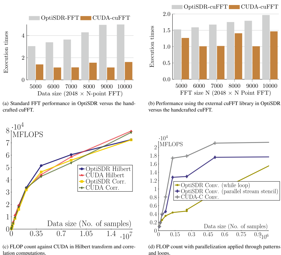
Fig. 5 Fourier and Hilbert transforms performance using OptiSDR and handcrafted CUDA
