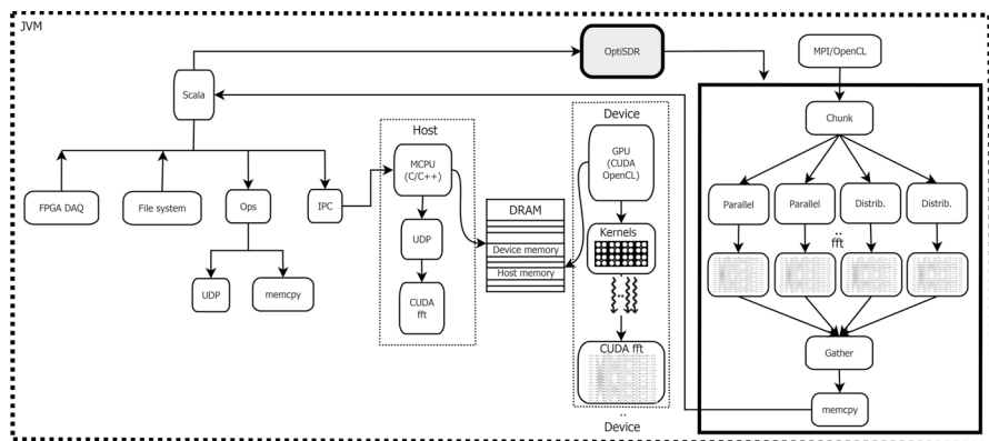
Fig. 1 The OptiSDR platform elements and interfaces. Besides GPUs and MCPU, the development methodology is agile to generate code from multiple GPLs for nodes of computer clusters due to compatibility with CUDA and MPI
