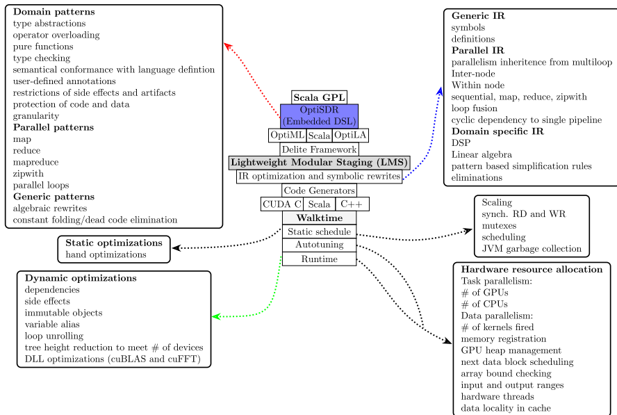
Fig. 3 OptiSDR framework, backend, and frontend layers and static/dynamic optimization steps using generic and domain-specific intermediate representations and tuning of the runtime. The framework achieves agility through the use of scaffold of libraries and staging by refining constructs late in the compilation
