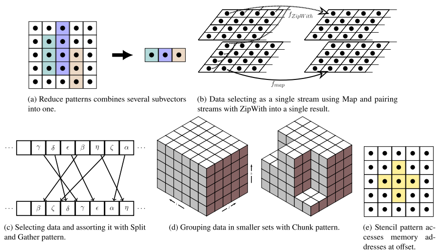
Fig. 2 Parallel patterns adopted in OptiSDR from the functional programming model. The patterns can be combined for complex signal processing tasks
