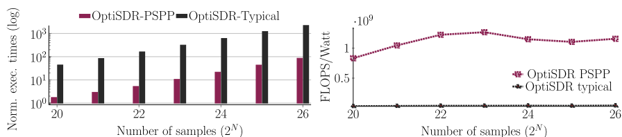
Fig. 9 Speed and wattage comparison with two OptiSDR implementations: PSPP versus Scala's top-down approach involving memory copying within JVM
