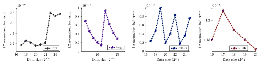
Fig. 7 Accuracy benchmarking of OptiSDR using different algorithms
