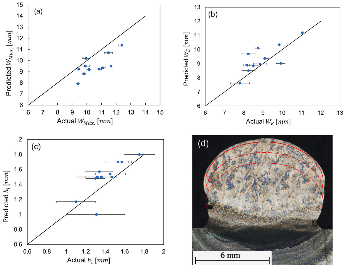
Fig. 10. Comparison of predicted and actual maximum wall width W_{Max} (a), effective wall width W_E (b) and layer height h_l (c) for PTA samples. The predicted bead shape (red line) for one typical case of PTA deposition using ER90S-G steel wire with an inter-layer temperature of 70 °C is superimposed in the etched macrograph (d). (For interpretation of the references to colour in this figure legend, the reader is referred to the web version of this article.)
