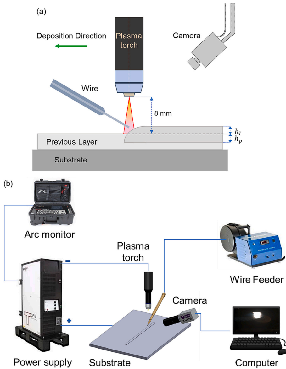
Fig. 8. (a) Schematic configuration of the PTA-based process (side view) for single-pass multi-layer straight wall deposition using ER90S-G steel wire, and illustration of the layer height h_l and penetration melting height h_p ; (b) Experimental setup of PTA deposition process and equipment.
