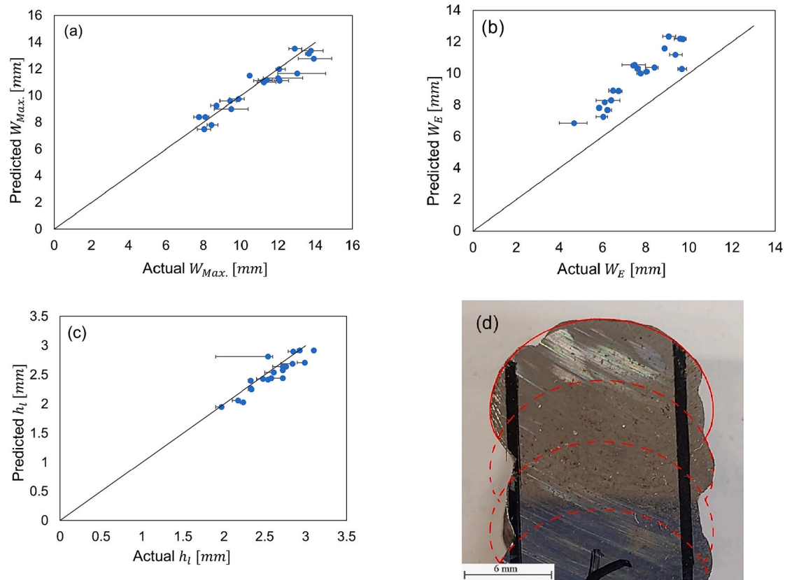
Fig. 11. Comparison of predicted and actual maximum wall width W_{Max} (a), effective wall width W_E (b) and layer height h_l (c) for CW-GMA samples. The predicted bead shape (red line) is superimposed in the cross-sectional macrograph for one typical case of CW-GMA deposition process (d). (For interpretation of the references to colour in this figure legend, the reader is referred to the web version of this article.)
