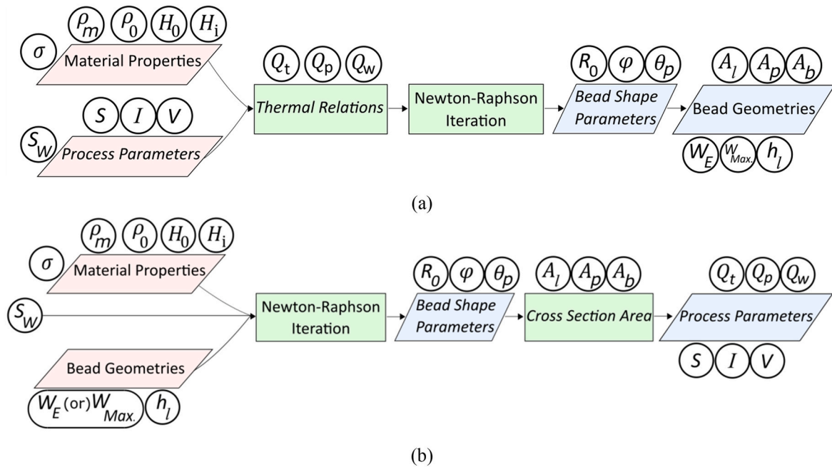
Fig. 6. (a) Flowchart of forward model for prediction of bead geometries; (b) Flowchart of reverse model for prediction of process parameters.
