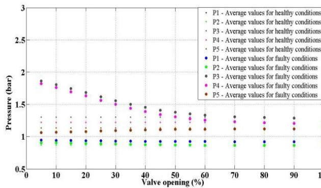
Fig. 8. Physical behavior – Clogged nozzle scenario
