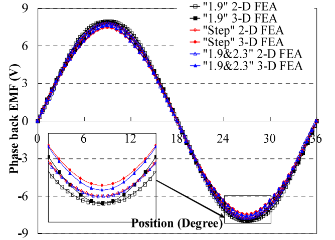
Fig. 8. Phase back EMF waveforms at 1000rpm with different rotor configurations from 2-D and 3-D FEA.
