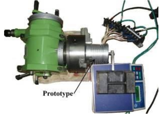
Fig. 16. Experimental setup.
