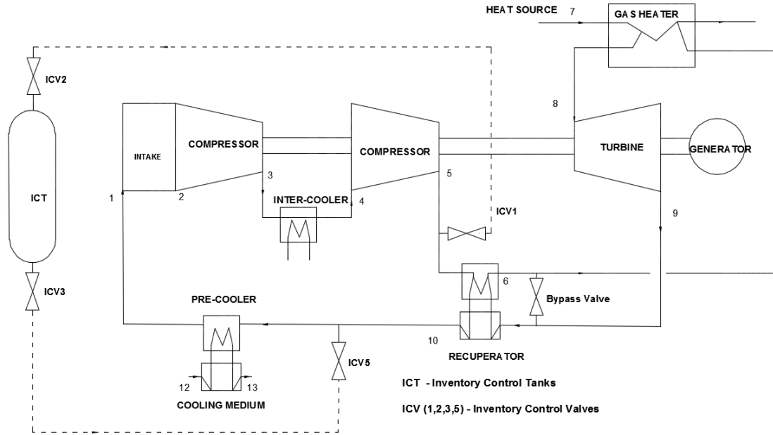
Figure 1: Scheme of Reference Plant Circuit with Different Control Options
