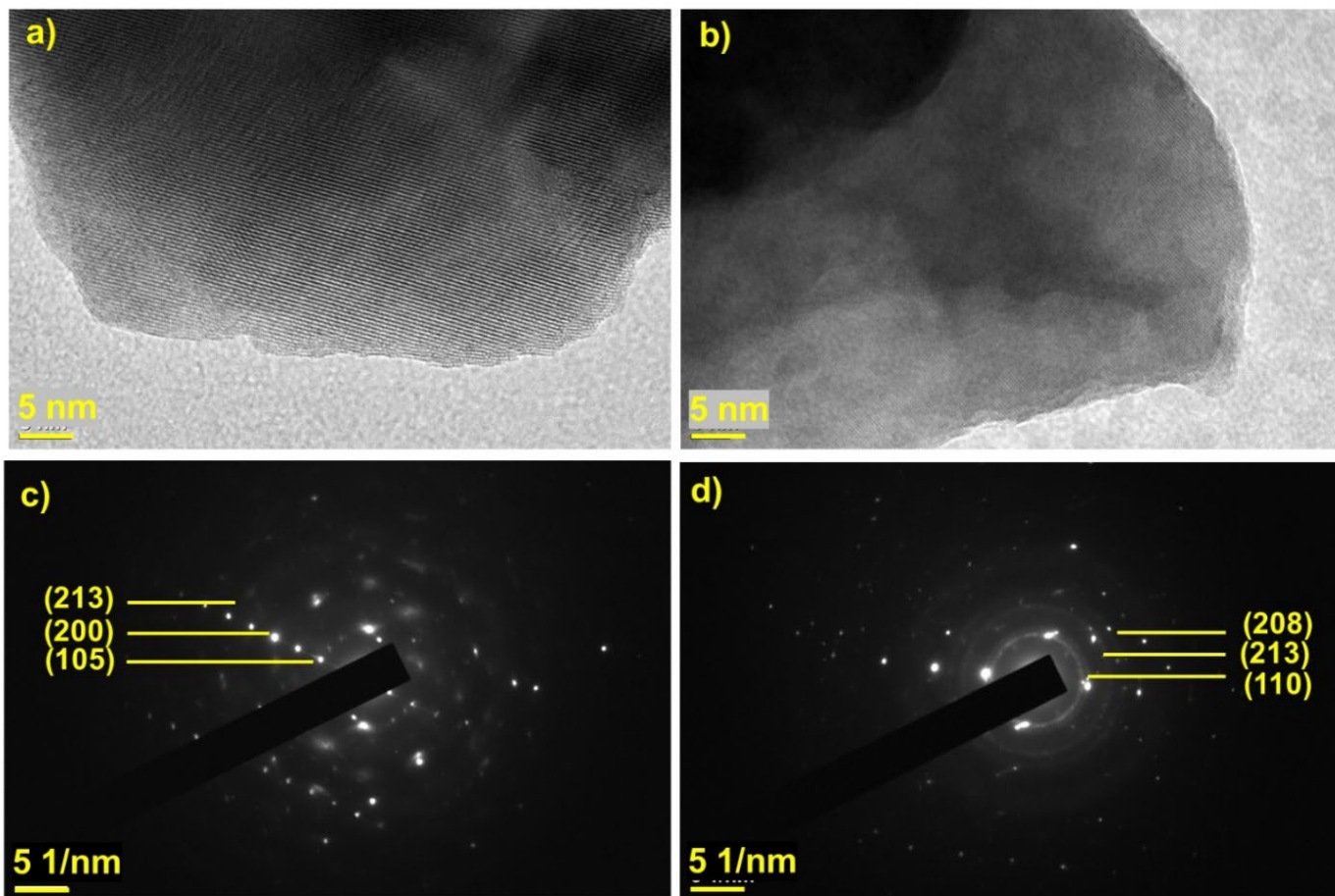
Figure 4: HRTEM images of (a) LPC-R and (b) LPC-2 with corresponding SAED patterns of (c) LPC-R and (d) LPC-2
