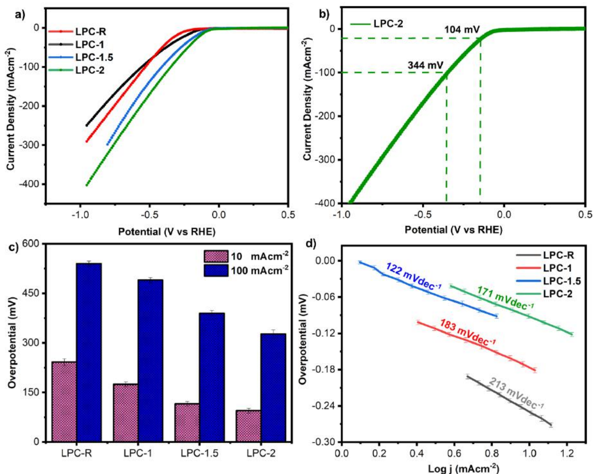
Figure 9: (a) HER polarization curves, (b) Reverse polarization curve of LPC-2, (c) Bar graph of overpotential at 10 and 100 \text{ mAcm}^{-2} , (d) Tafel plot.
