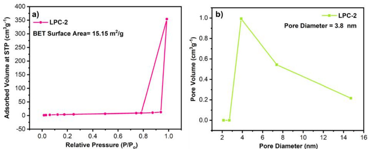
Figure 6: (a) N 2 adsorption-desorption isotherms of LPC-2. (b) Pore size distribution curves of LPC-2.
