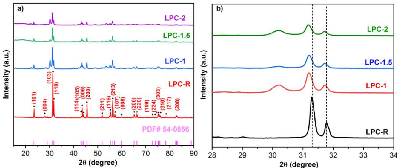
Figure 2: (a) p-XRD Diffractograms of LPC-R, LPC-1, LPC-1.5, and LPC-2, which show a close comparison to \text{La}_{0.95}\text{Pr}_{1.05}\text{CuO}_4 (JCPDS 54-0856). (b) Magnified representative 2\theta region showing the peak shifts in (103) and (110).
