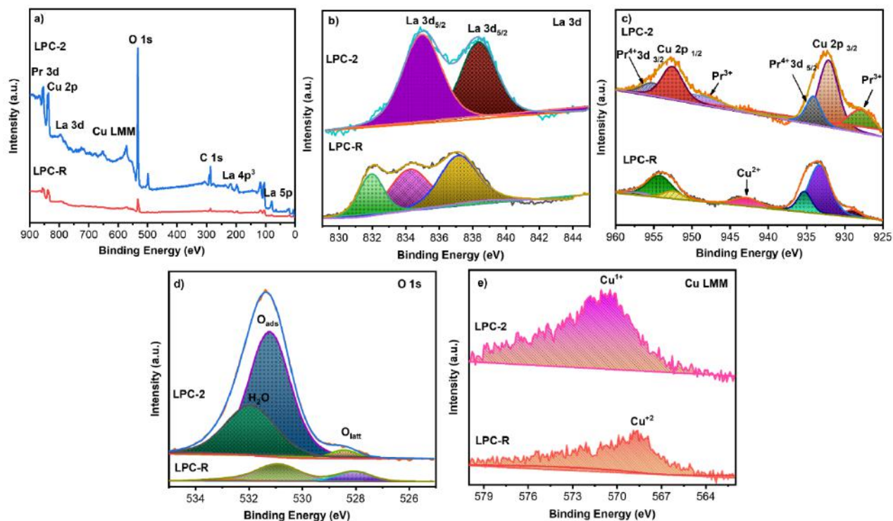
Figure 7: XPS analysis of LPC-R and LPC-2: (a) survey scan, (b) high-resolution spectra of La 3d (c) high-resolution spectra of Cu 2p and Pr 3d, (d) O 1s spectra, (e) Cu LMM Auger peaks.
