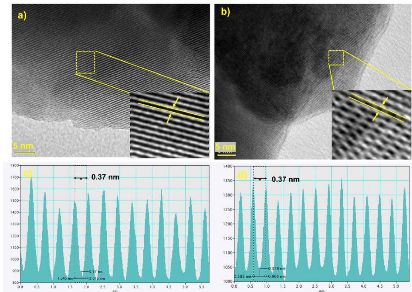
Figure 5: (a) HRTEM image of LPC-R with the inset showing the corresponding inverse FFT. (b) HRTEM image of LPC-2 with an inset showing the corresponding inverse FFT. (c-d) Profile graphs of the insets in (a) and (b).
