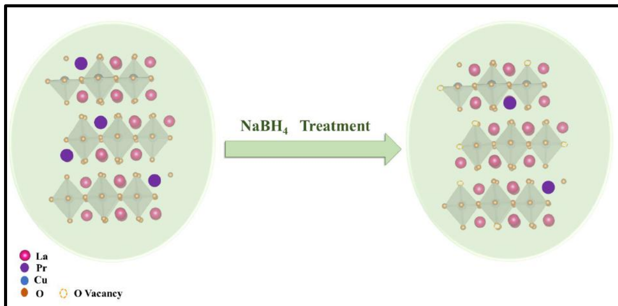
Figure 1: Surface Reconstruction of \text{La}_{0.95}\text{Pr}_{1.05}\text{CuO}_4
