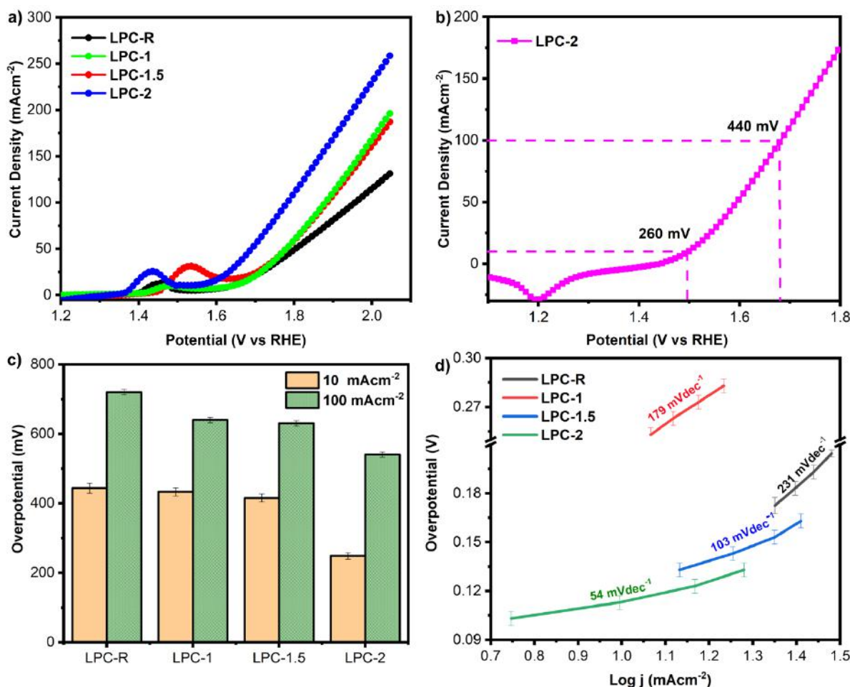
Figure 8: (a) OER polarization curves, (b) Reverse polarization curve of LPC-2, (c) Bar graph of overpotential at 10 and 100 \text{mAcm}^{-2} , (d) Tafel plot.
