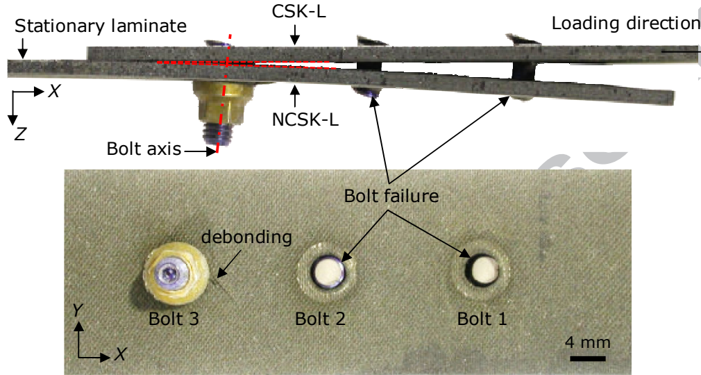
Figure 6: Combination of bearing and bolt failure in three-bolt CBJ
