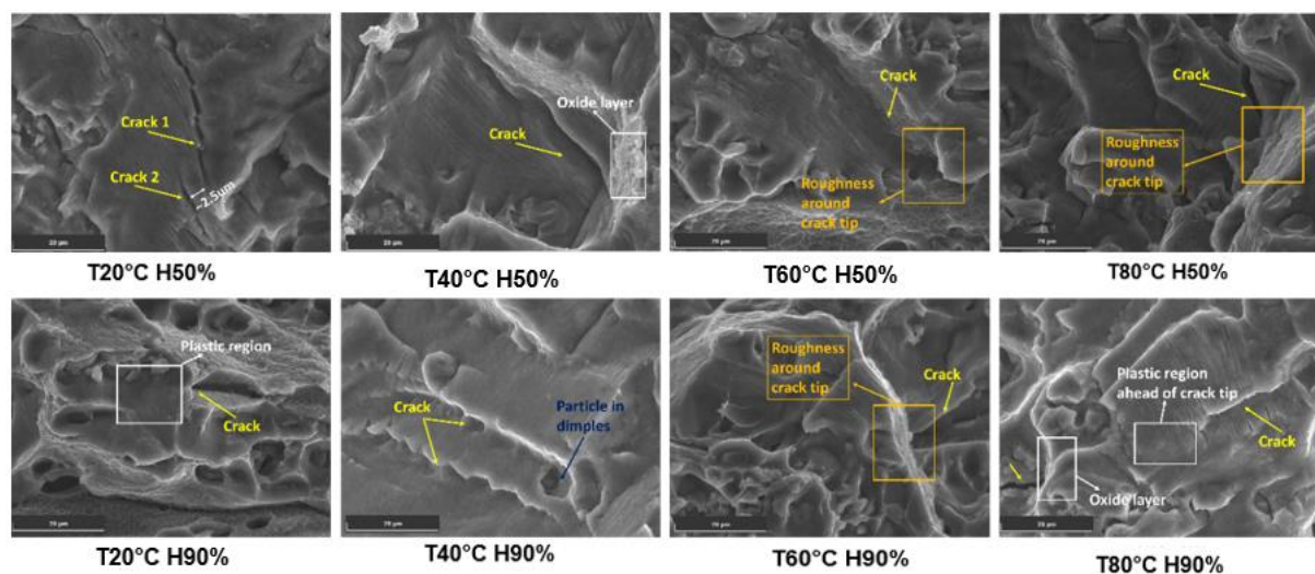
Figure 6. Crack closure mechanisms observed in different conditions. Scale bar 20 \mu\text{m} .
