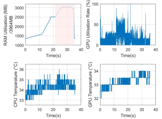
Fig. 10. GRU operation performance on Jetson Nano.
