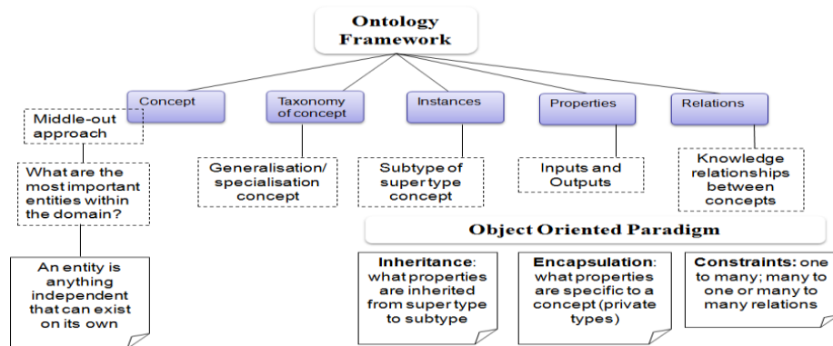
Figure 3. Object Oriented Paradigm way of thinking into Ontology Development
