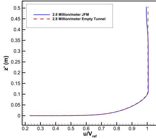
(a) Full profile for BL
