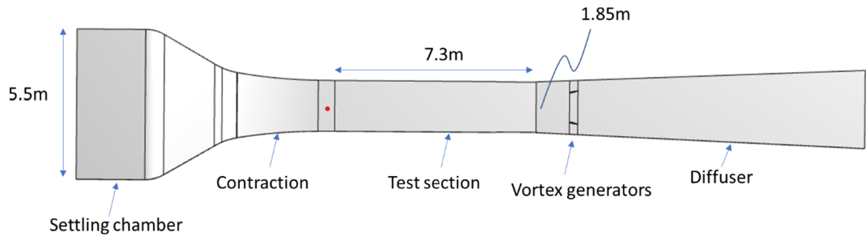
(b) Nominal geometry of the high-speed leg of VTSWT
