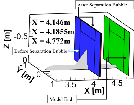
(a) Extraction locations
