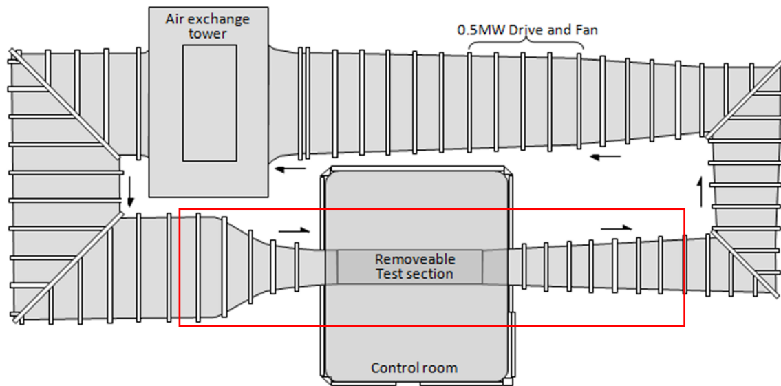
(a) Top-view schematic of the Virginia Tech Stability Wind Tunnel. Red box highlights the high speed leg shown in figure 2b
