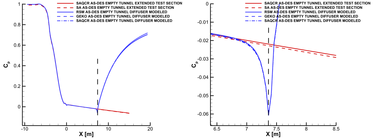
(a) Streamwise C_p distribution along the port side-wall centerline. (b) Streamwise C_p distribution along the port side-wall centerline. Zoomed in at diffuser inlet ( x \approx 7.355 m).
