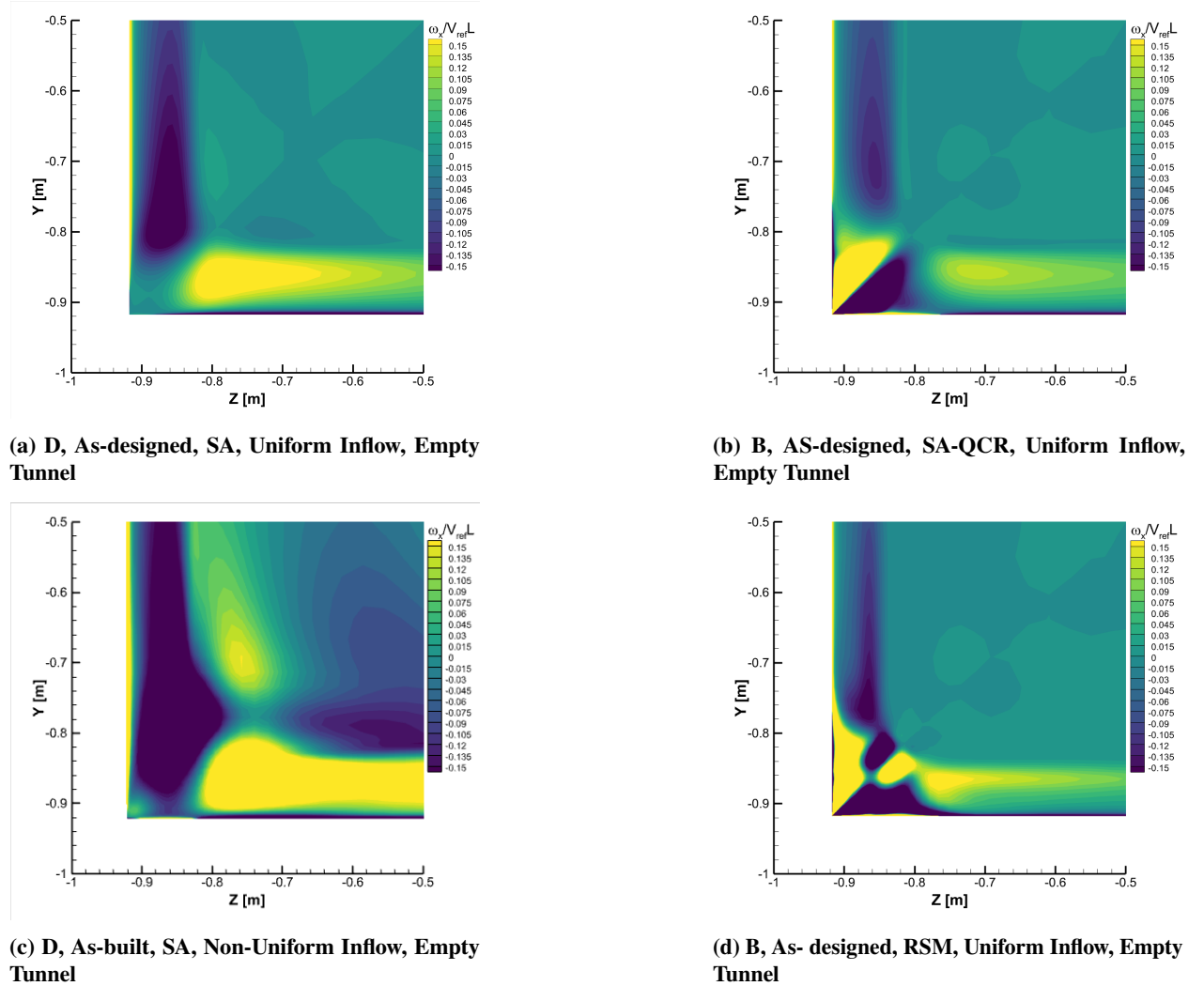
Fig. 9 Streamwise vorticity contour at the port-floor corner, x = 3.26 m, Re = 2.8 M/m.
