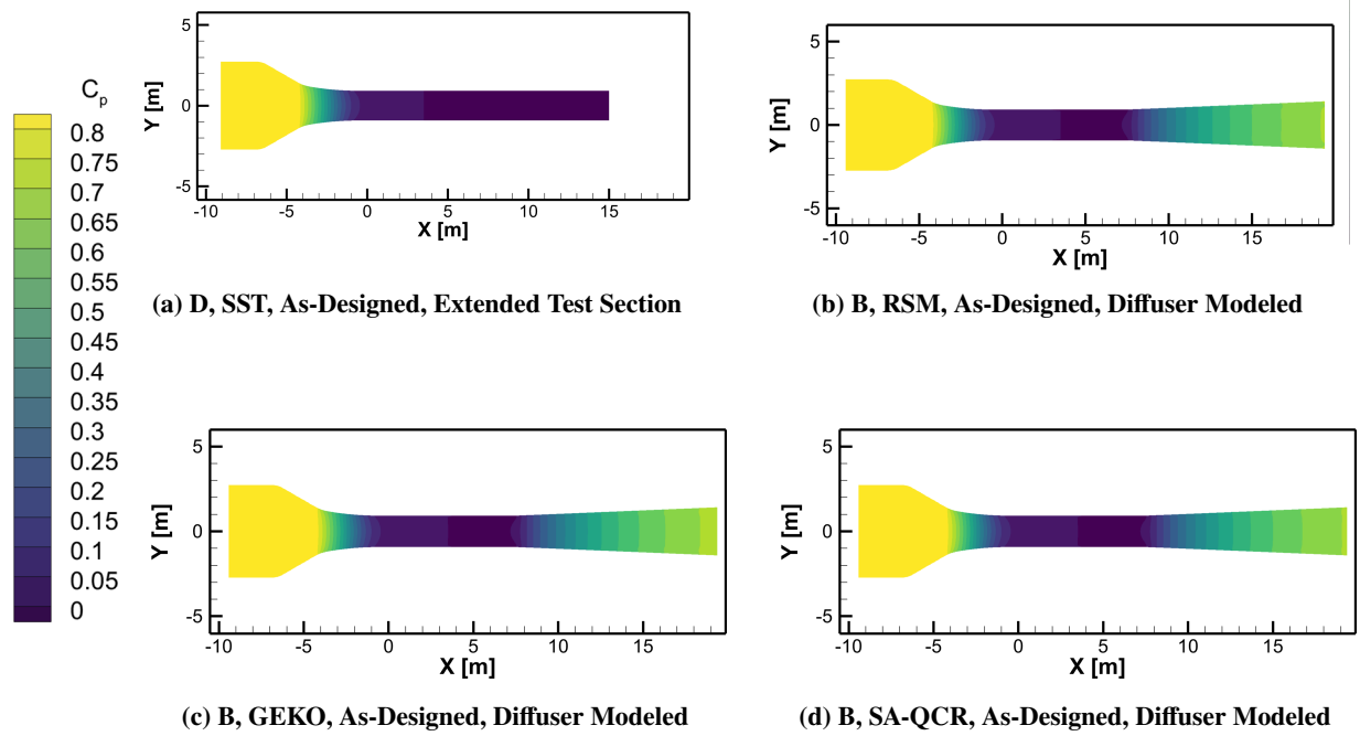
Fig. 20 Centerplane C_p contours at Re = 3.9 Million/meter. D as-designed extended test section simulation compared with B diffuser modeled simulations.
