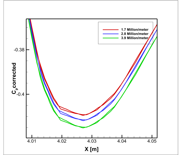
(b) z = -0.214 m, leading-edge detail
