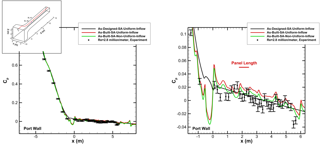
(a) C_p distribution zoomed to show settling chamber, contraction and test section.
