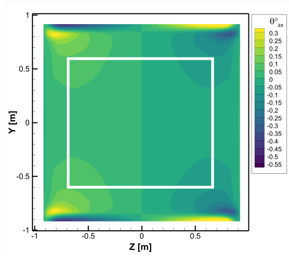
(b) As-Designed Uniform Inflow
