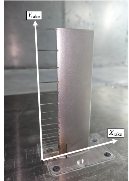
(d) Floor-mounted boundary-layer rake, close-up view.
