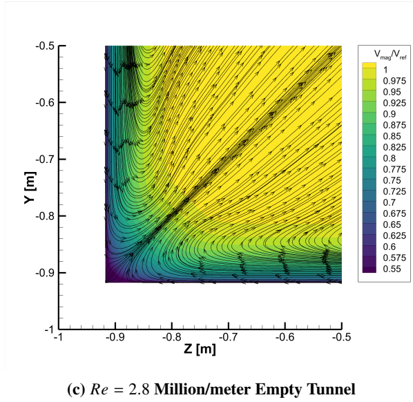
Fig. 29 Submission D as-designed model-in and empty-tunnel case. Velocity magnitude contour downstream of the model at x = 5.0888 m. The streamline overlay highlights the in-plane streamlines.
