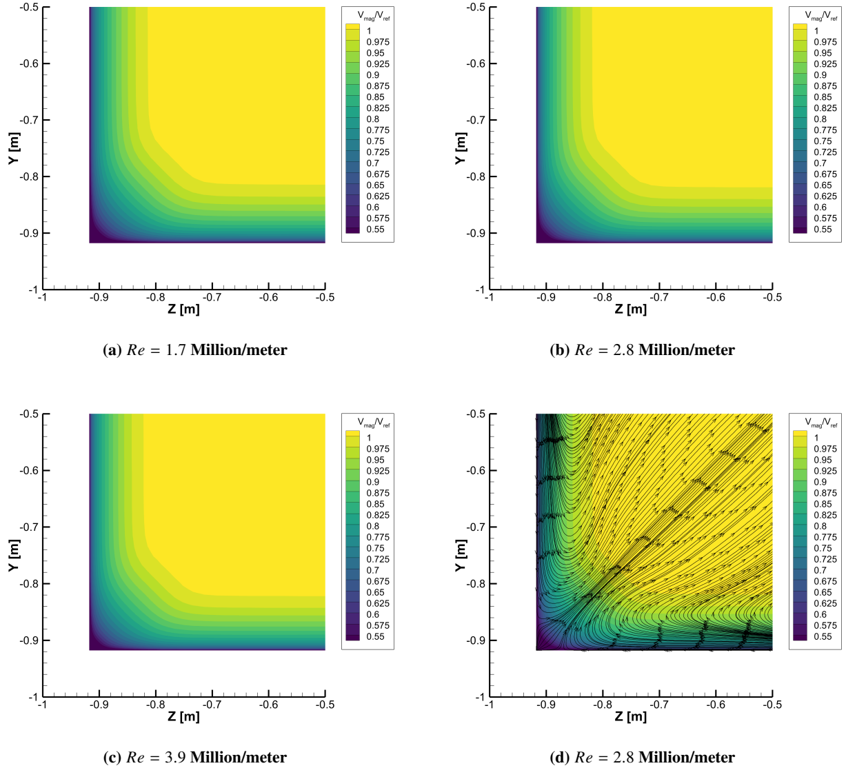
Fig. 24 Submission D as-designed model-in. Velocity magnitude contour downstream of the model at x = 5.0888 m, across three Reynolds numbers. The streamline overlay at Re = 2.8 Million/meter highlights the in-plane streamlines.
