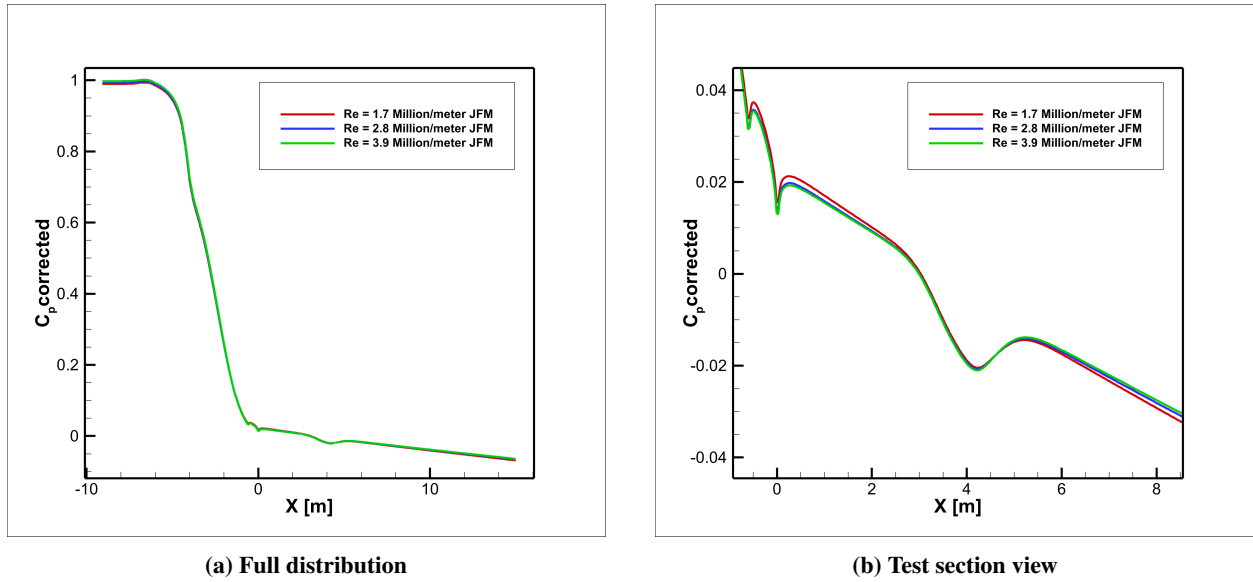
Fig. 27 Reynolds number effects on the pressure coefficient along the centerline of the starboard wall.
