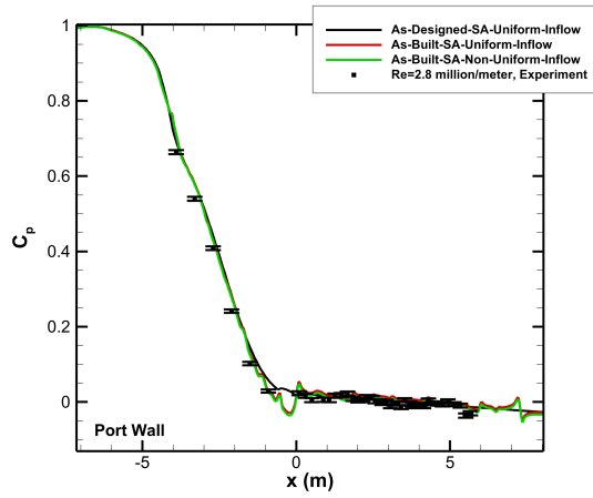
(c) C_p at port wall centerline
