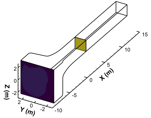
(b) Inflow plane and measured contour extraction plane ( x = 3.26 m).
