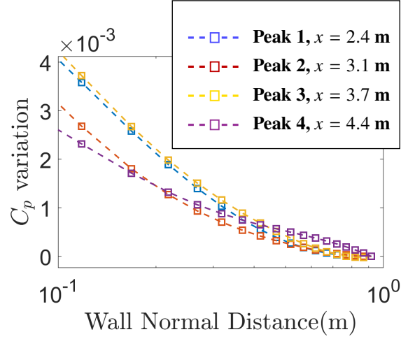
(b) Magnified view of the wall-induced C_p peak across the same spanwise stations in (a), illustrating the exponential decay with distance from the wall.
