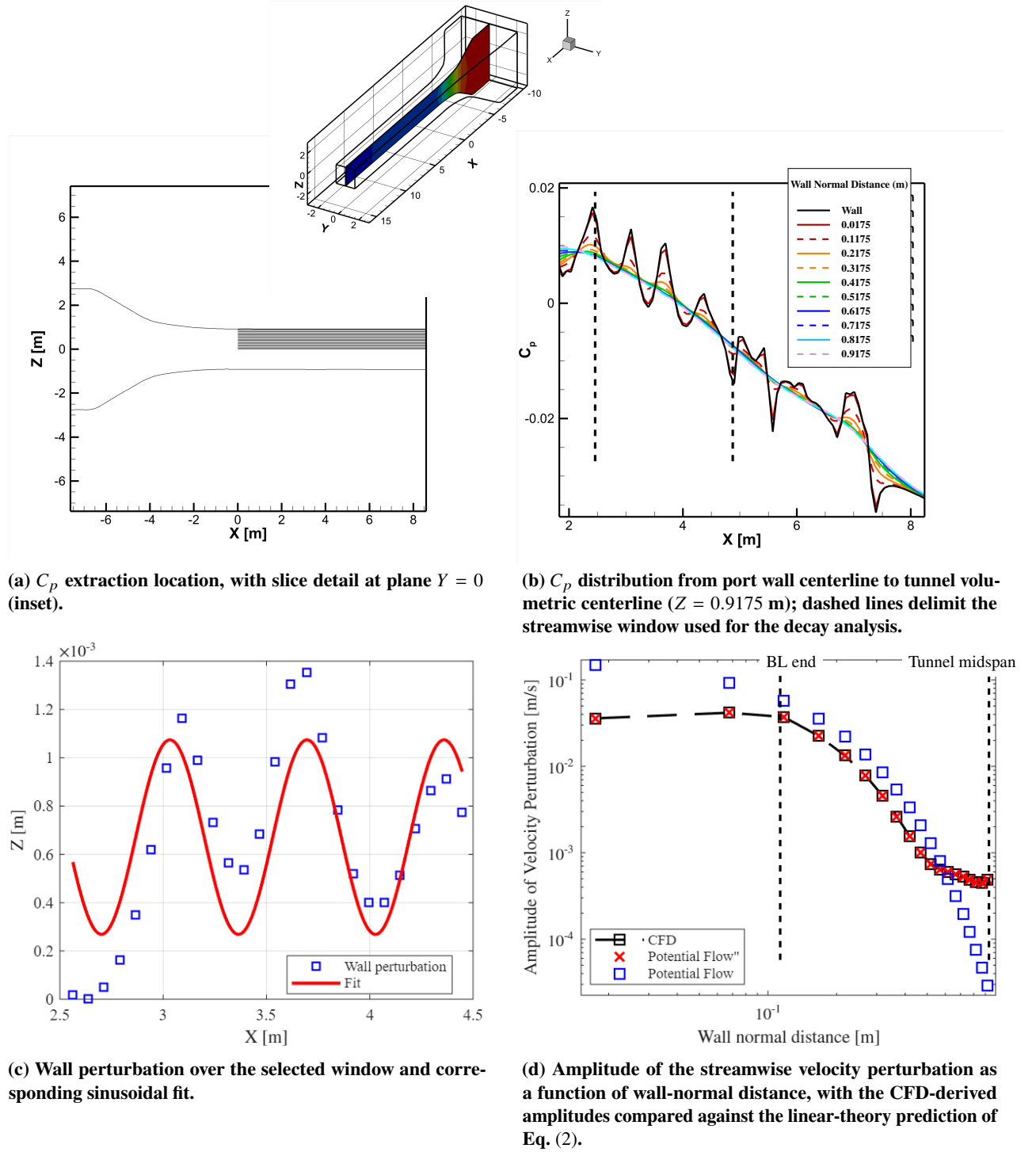
Fig. 19 Potential flow pressure decay analysis for as-built VTSWT walls.
