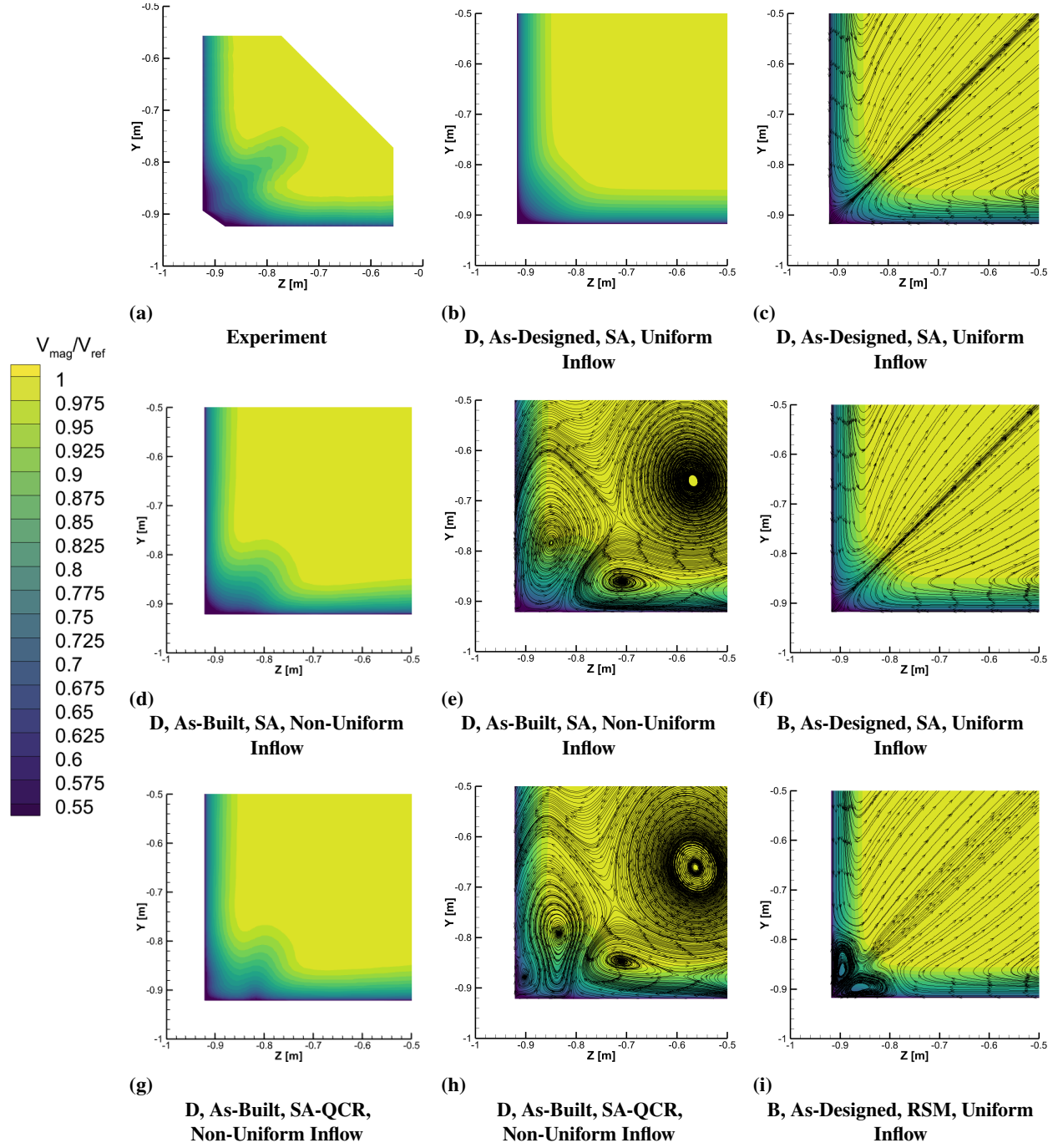
Fig. 17 Contour plots of velocity magnitude at the reference location ( x = 3.26 \text{ m} ) zoomed in to the starboard-floor corner. Contour plots are shown for Re = 2.8 \text{ Million/meter} , empty tunnel case.
