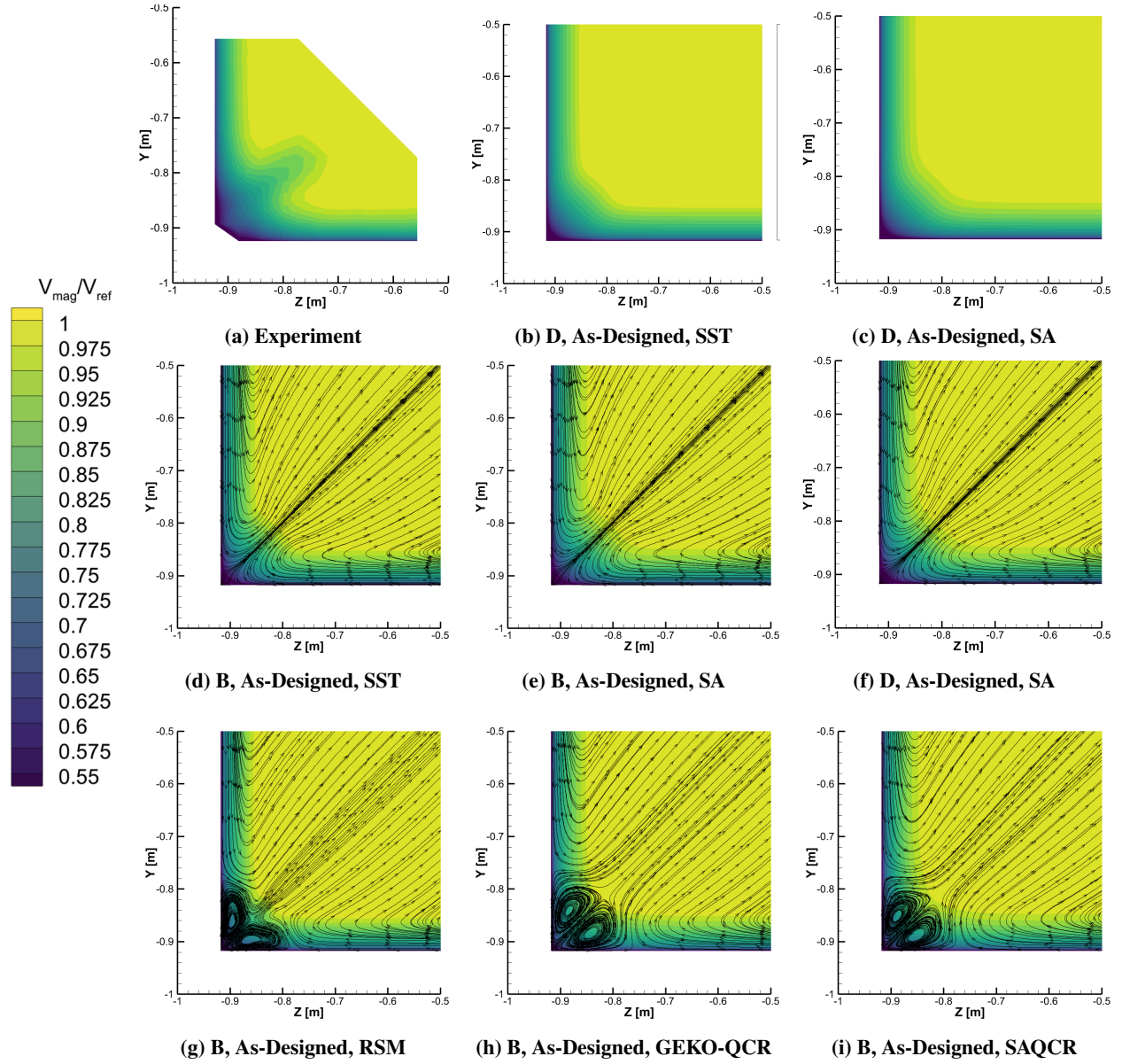
Fig. 16 Contour plots of velocity magnitude at the reference location ( x = 3.26 m) zoomed in to the starboard-floor corner. Contour plots are shown for Re = 2.8 Million/meter, uniform inflow, empty tunnel case.
