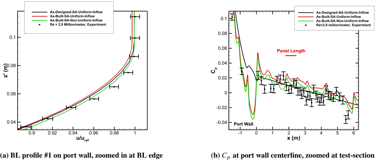
Fig. 11 Port-side boundary layer profile and pressure coefficient distribution, zoomed views. z' represents the wall-normal distance for the BL extraction.
