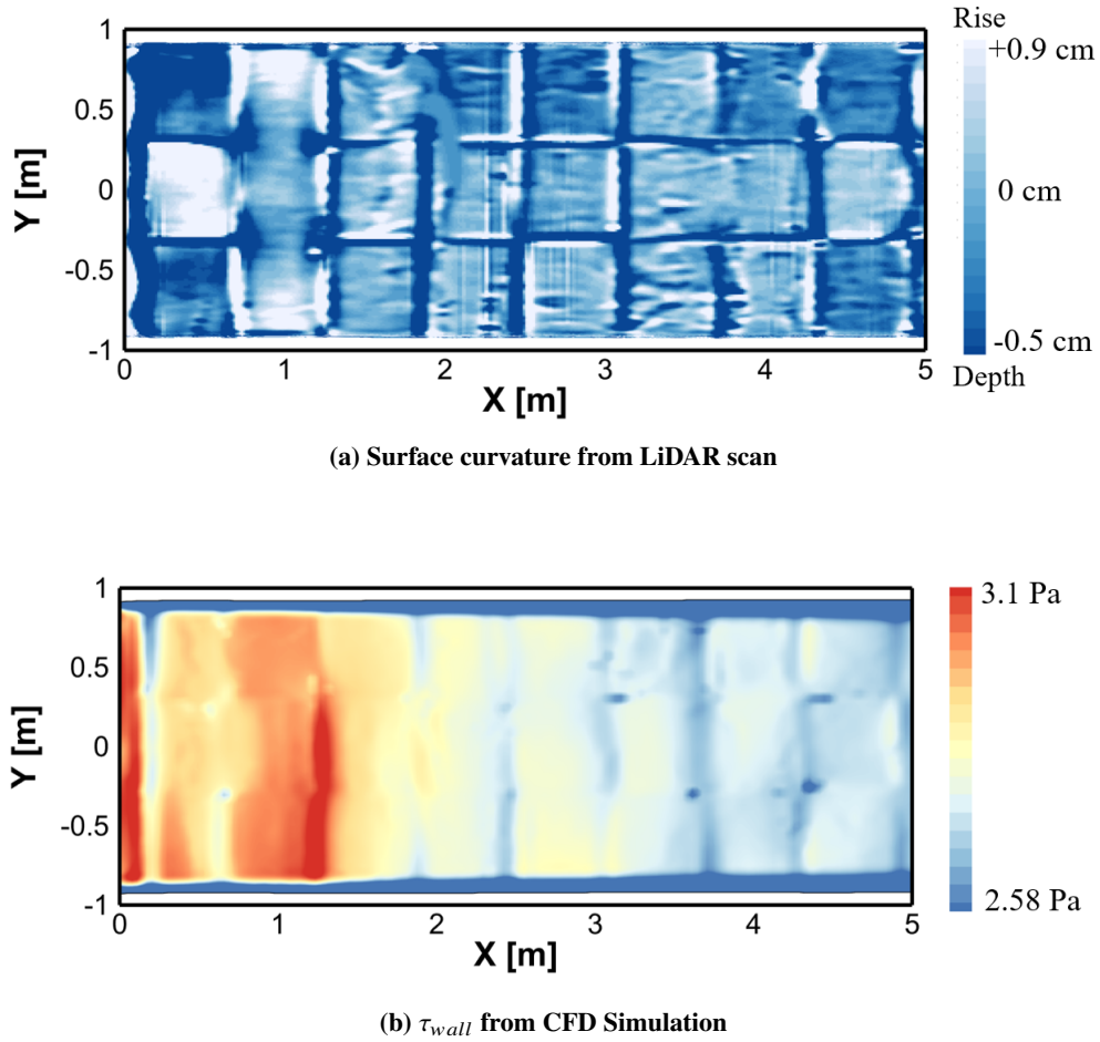
Fig. 1 Surface curvature and flow behavior on VTSWT's port side test-section wall
