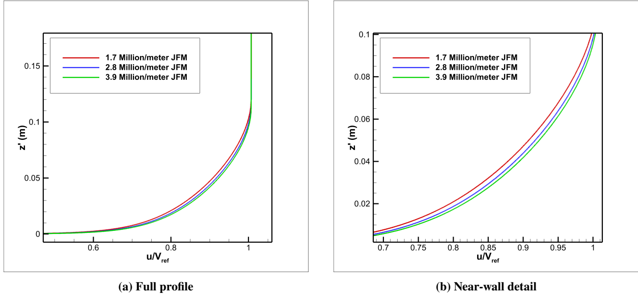
Fig. 26 Reynolds number effects on the boundary layer profile at x = 5.0888 m.
