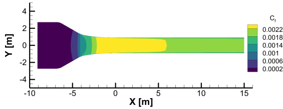
(b) Re = 3.9 Million/meter, D, As-Designed, SA, Uniform Inflow, Empty Tunnel.
