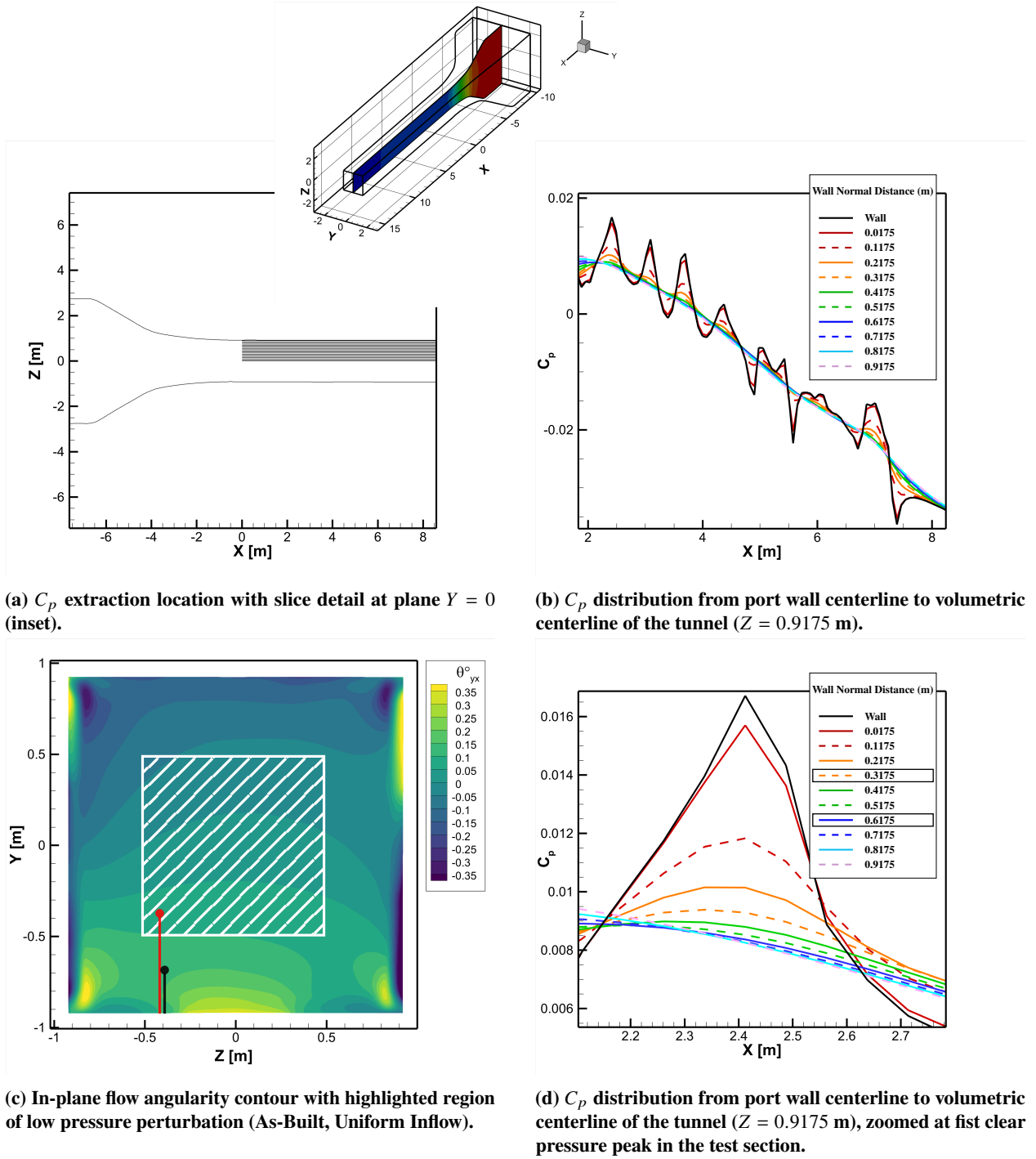
Fig. 10 Pressure perturbation analysis for the as-built empty tunnel configuration.
