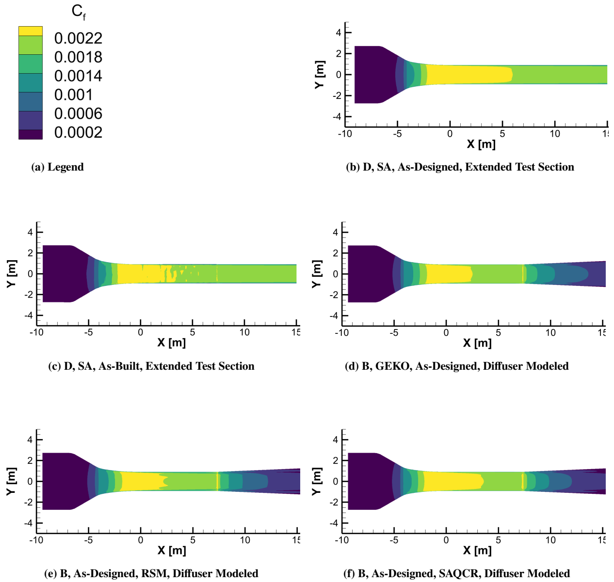
Fig. 22 Contour plots of skin friction coefficient on the tunnel port wall.
