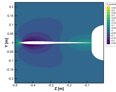
(i) Re = 3.9 Million/meter, x = 4.1855 m
