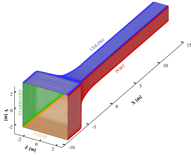
(a) CFD coordinate system.
