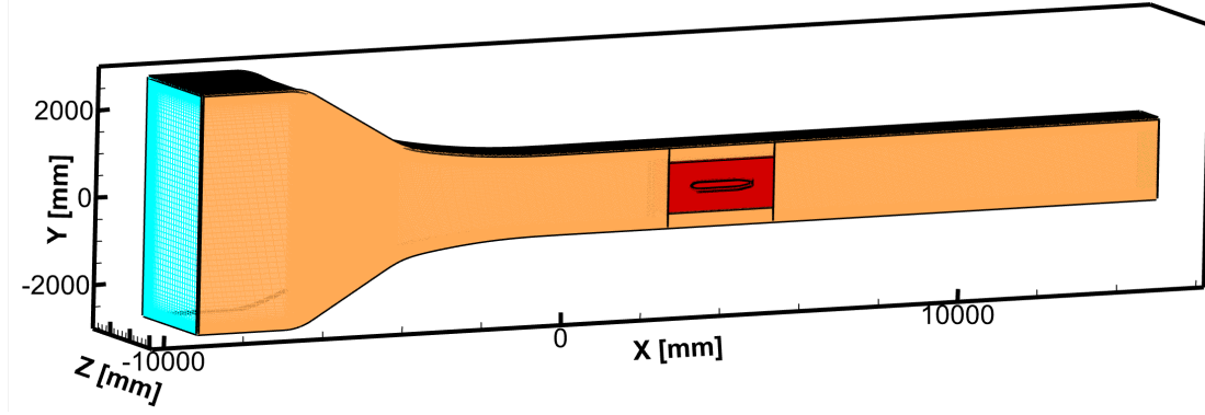
(a) Level 5 VTSWT and JFM model-in grid. The orange-highlighted region denotes the VTSWT tunnel block, and the red region represents the JFM block. Both orange and red regions correspond to symmetry boundary conditions. The blue region indicates the inlet plane.
