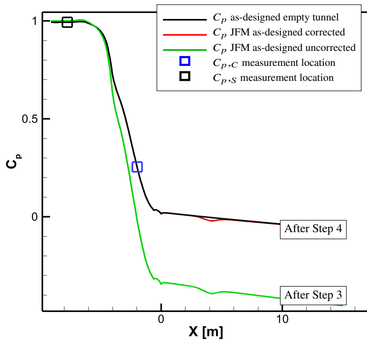
Fig. 32 Effect of the empty-tunnel calibration on the model-in C_p distribution. The corrected curve references the model-in pressure to the freestream condition established by the empty-tunnel calibration, enabling direct comparison with experimental data.
