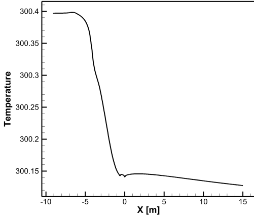
(a) Temperature variation at port wall centerline, Re = 3.9 Million/meter, D, As-Designed, SST, Uniform Inflow, Empty Tunnel.
