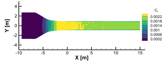
(c) Re = 3.9 Million/meter, D, As-Built, SA, Uniform Inflow, Empty Tunnel.
