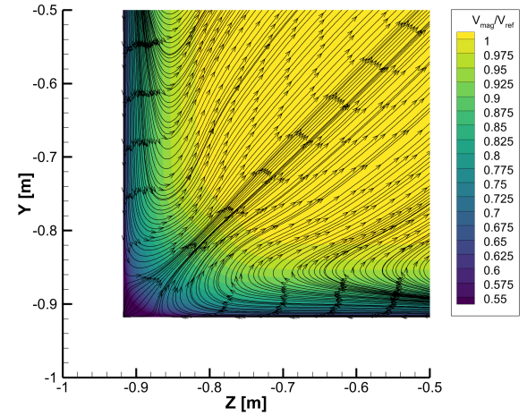
Fig. 29 Submission D as-designed model-in and empty-tunnel case. Velocity magnitude contour downstream of the model at x = 5.0888 m. The streamline overlay highlights the in-plane streamlines.
