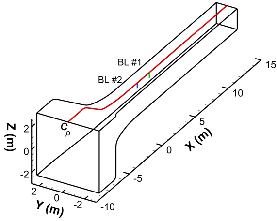
(a) Extraction locations for C_p and boundary layers on the port side wall. C_p measurements are repeated similarly for the starboard wall, and boundary layer measurements are repeated on all four walls.
