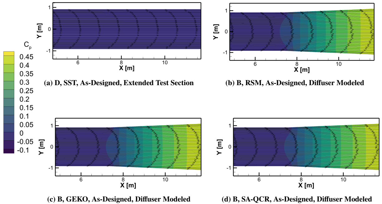
Fig. 21 Zoomed centerplane C_p contours at Re = 3.9 Million/meter. D as-designed extended test section simulation compared with B diffuser modeled simulations.
