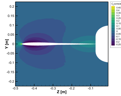
(c) Re = 1.7 Million/meter, x = 4.1855 m
