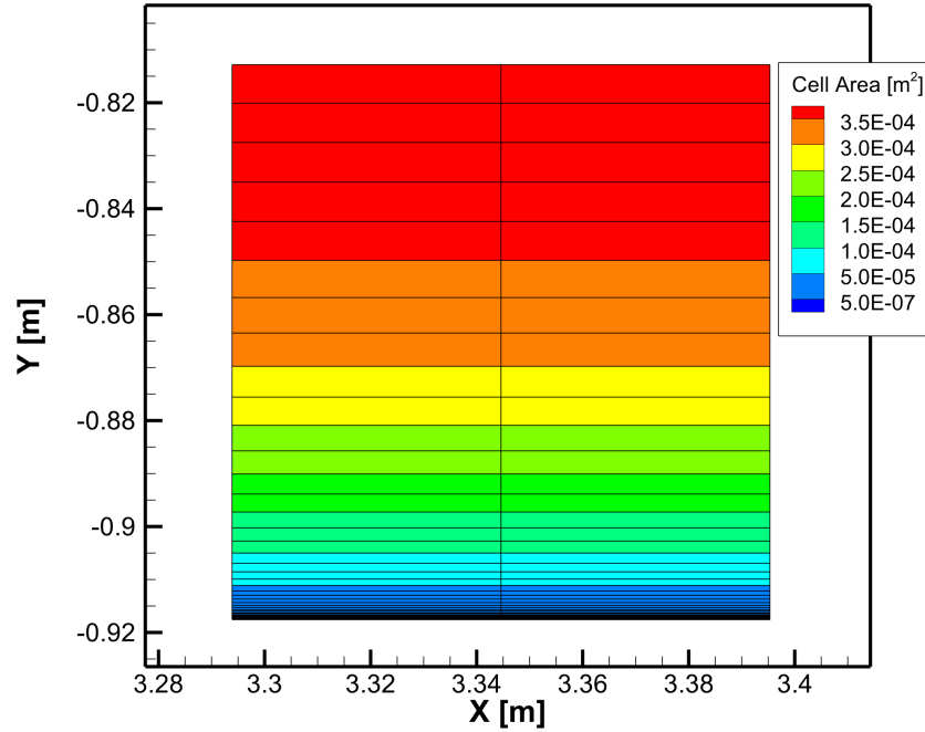
Fig. 15 Wall-normal grid distribution through the test-section boundary layer at the Level 7 of the empty-tunnel grid family, showing near-wall point clustering and cell density maintained through the boundary-layer edge.
