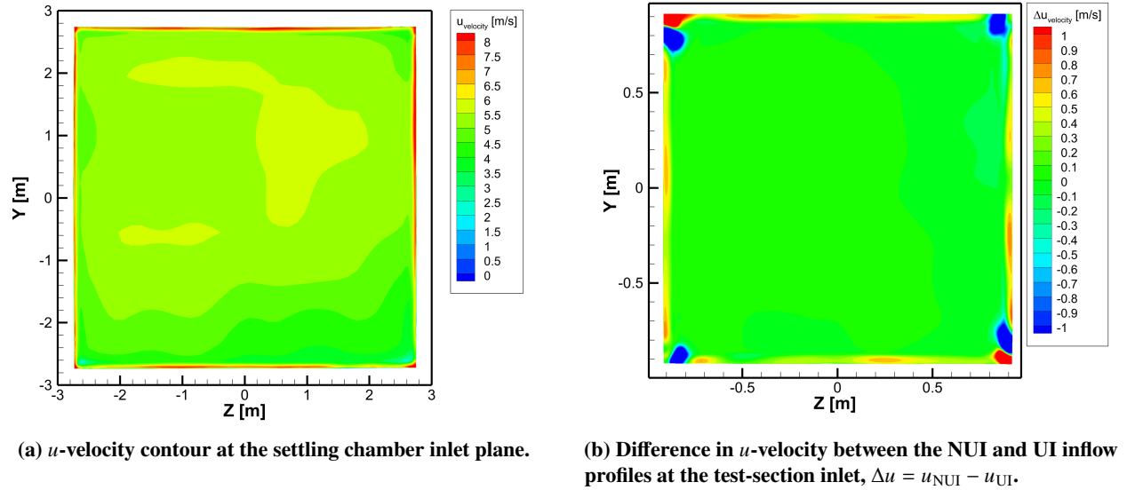
Fig. 5 Inflow characterization for Re = 3.9 Million/meter. (a) Measured non-uniform inflow profile prescribed at the CFD domain inlet. (b) Difference between the non-uniform and uniform inflow profiles at the test-section inlet, illustrating the near-wall acceleration delivered by the non-uniform inflow condition.
