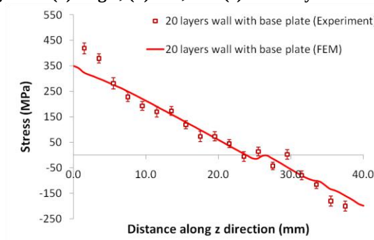
Fig. 10: Longitudinal stress along the normal direction of the mid-section in the deposited wall.
