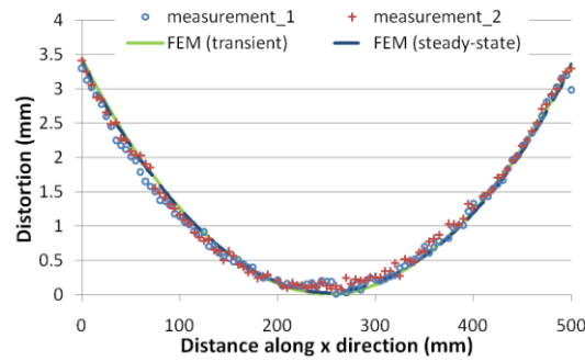
Fig. 8: Distortion verification along the longitudinal direction after the clamps were removed.
