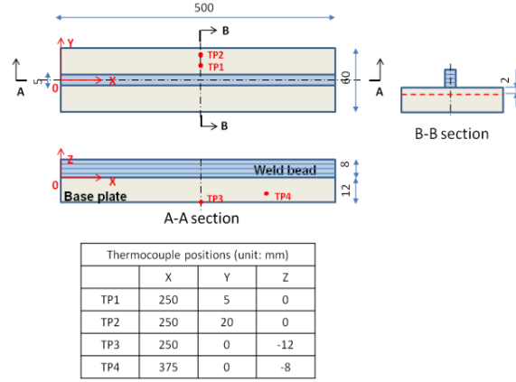
Fig. 2: Geometry of the WAALM sample.
