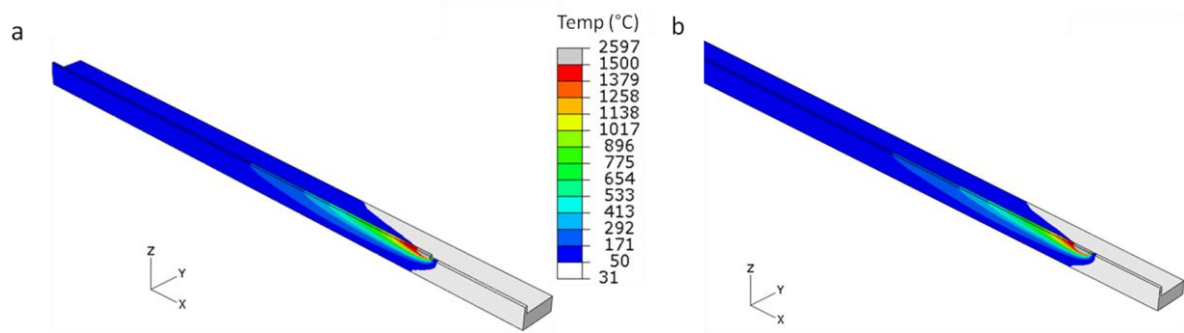
Fig. 5: Temperature distribution from: (a) transient and (b) steady-state thermal models.
