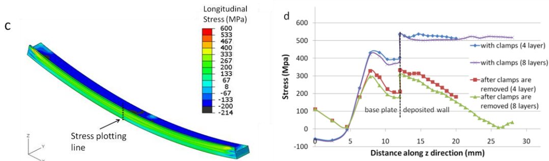
Fig. 7: Longitudinal residual stress predictions from: (a) transient thermal and mechanical models; (b) steady state thermal and mapped mechanical models; (c) steady state thermal and mapped mechanical models after clamps were removed (a scaling factor of 5 is used for the distorted shape); and (d) the stress plotted along the lines shown in of (b) and (c).
