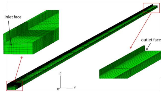
Fig. 4: Mesh of the steady state thermal model.
