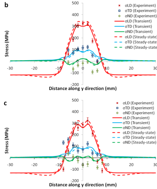
Fig. 9: Stresses in the longitudinal (LD), transverse (TD) and normal (ND) directions along a transverse line in the base-plate indicated in Fig. 2 for (a) single, (b) two, and (c) three layers.
