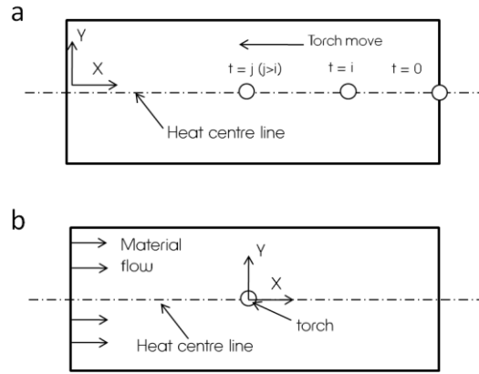
Fig. 1: Model with different reference frames. (a) Lagrangian reference frame (b) Eulerian reference frame.
