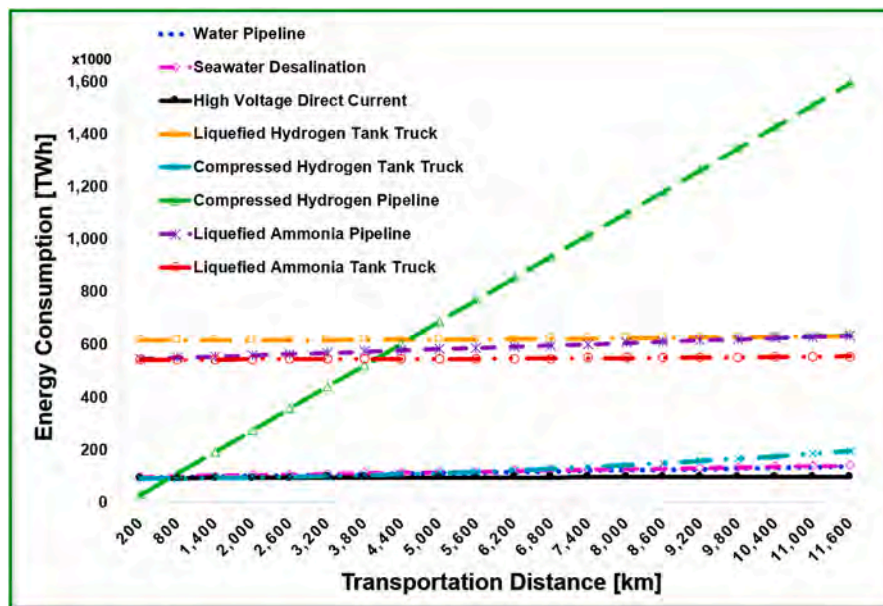
Fig. 16. Sensitivity analysis of energy consumption with varying transportation distance at a fixed exploitable solar PV electricity generation of 50% for high voltage direct current, water pipeline, seawater desalination, and liquefied hydrogen tank truck, compressed hydrogen pipeline, liquefied ammonia pipeline, liquefied ammonia tank truck, and compressed hydrogen tank truck systems.
