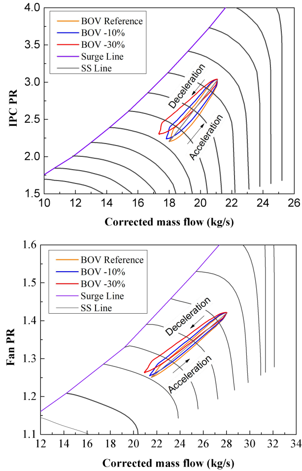
Fig. 14 IPC and Fan operating lines comparison.
