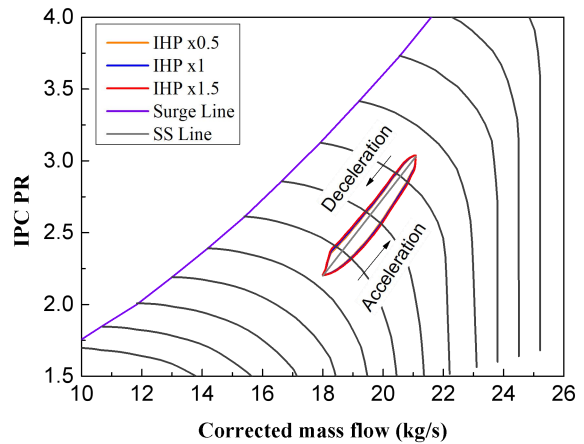
(b) HP shaft inertia influences
