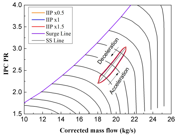
(a) IP shaft inertia influences
