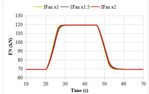
(b) FN comparison
