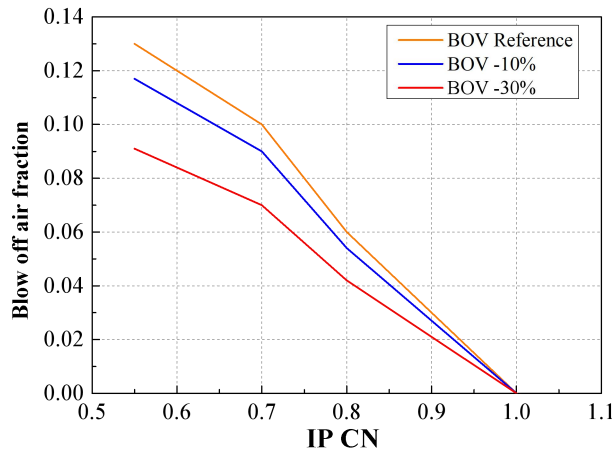
Fig. 4 BOV investigation cases.
