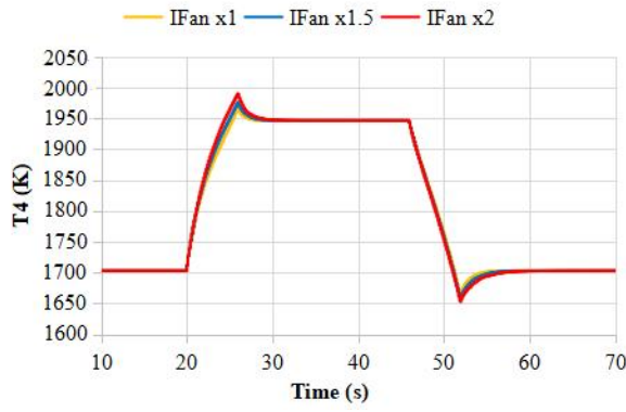
(a) T4 comparison
