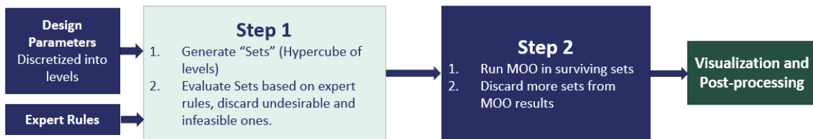
Figure 1. ADOPT Flowchart
