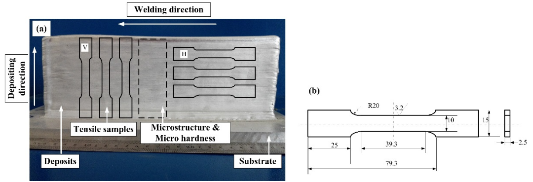
Fig.3. (a) The sampling positions of each wall; (b) the size of tensile sample
