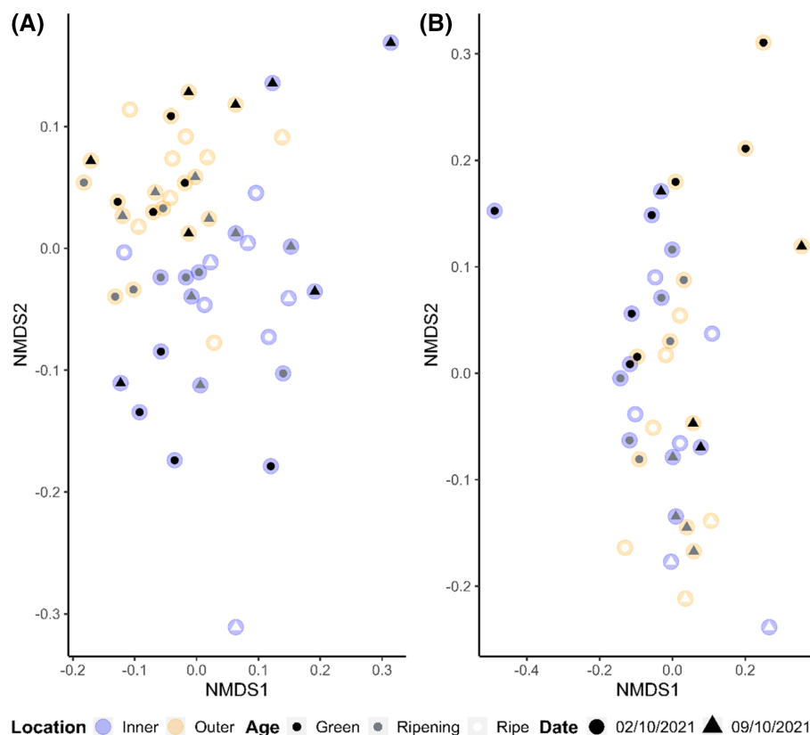
FIGURE 4 The first two dimensions of the NMDS analysis based on Bray–Curtis indices for (A) fungi and (B) bacteria from the surface of raspberries collected on two dates (2 October 2021 and 9 October 2021), from two locations within polytunnels (inner vs. outer) and across three ripening stages (green, ripening and ripe).
