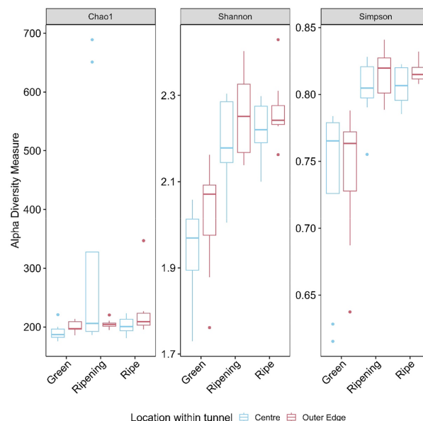
FIGURE 2 The alpha diversity measures for fungal Amplicon Sequence Variants (ASVs) of Chao1, Shannon and Simpson diversity indices. Four polytunnels were sampled across two repeats in time (2 October 2021 and 9 October 2021). The x-axis denotes fruit ripeness, and colour denotes location within the polytunnel.
