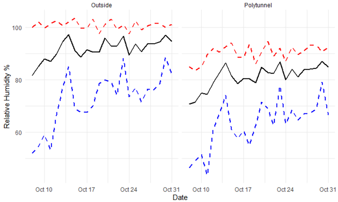
FIGURE A9 The average (black line), maximum (red line) and minimum (blue line) relative humidity from inside a polytunnel and in the outdoor air collected from dataloggers near the Rotorod samplers.
