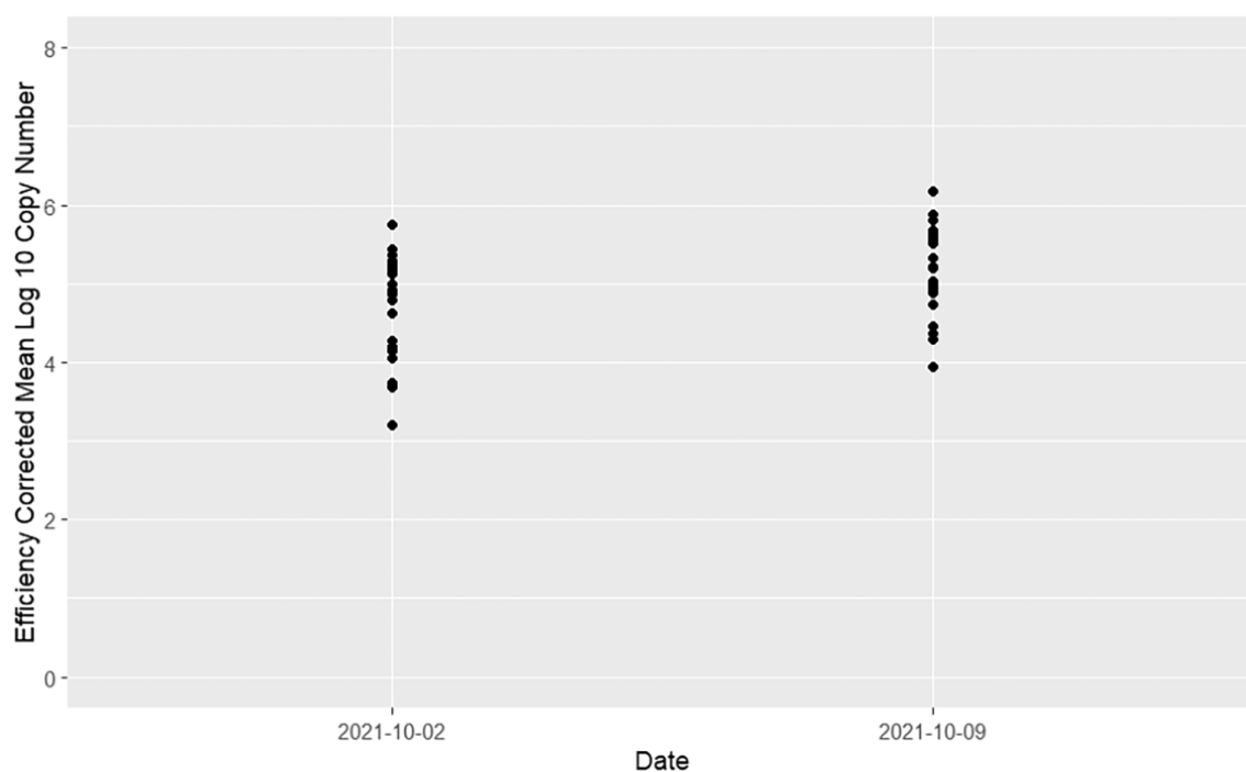
FIGURE A1 The efficiency corrected mean Log 10 copy number quantitative PCR results for the ITS of fungal epiphytes on the surface of raspberries across the two sampling dates.
