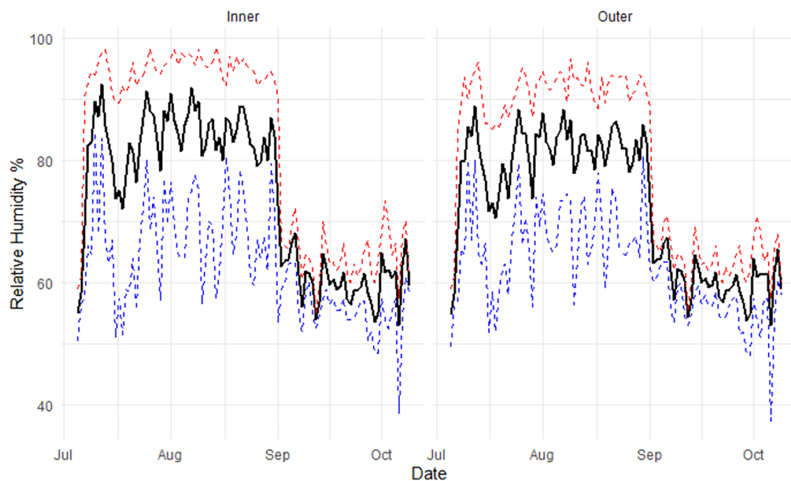
FIGURE A8 The average weekly humidity from the outer edge and centre of a polytunnel, the first samples were taken on 2 October 2021 and the second set of samples were taken on 10 October 2021.
