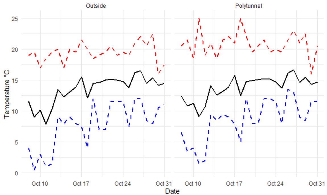
FIGURE A10 The average (black line), maximum (red line) and minimum (blue line) temperatures (°C) from inside a polytunnel and in the outdoor air collected from dataloggers near the Rotorod samplers.
