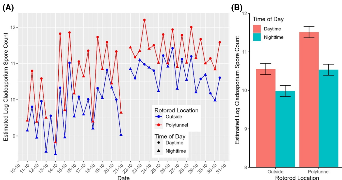
FIGURE 5 (A) The estimated Log Cladosporium spore count and (B) the estimated Log Cladosporium spore count averaged over location and time of day from spores collected using a Rotorod sampler from the centre of a polytunnel and in an open field over the day (08:00–20:00) and night (20:00–08:00) across 21 days in October 2022.
