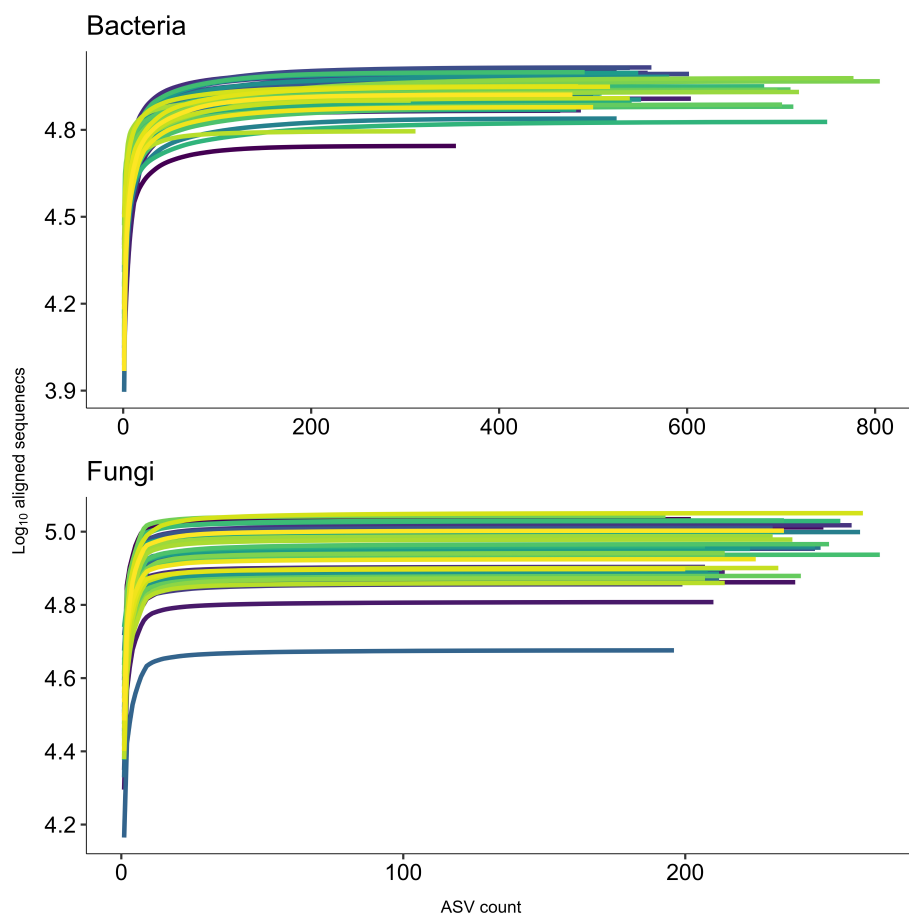
FIGURE A3 Rarefaction curves of log 10 ASV counts of fungal and bacterial ASVs.
