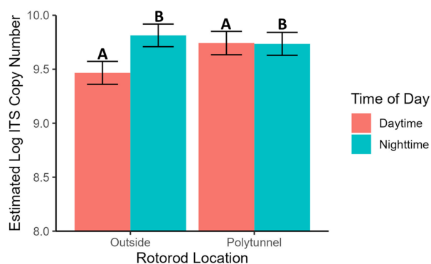
FIGURE A5 The estimated Log ITS copy number from airborne inoculum collected using a Rotorod sampler from the centre of a polytunnel and in an open field over the day (08:00–20:00) and night (20:00–08:00) across 21 days. Letters indicate significant differences between factor levels ( p < 0.05 ).
