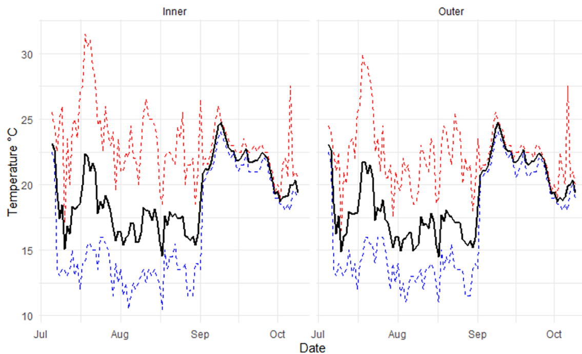
FIGURE A7 The average weekly temperature from the outer edge and centre of a polytunnel, the first samples were taken on 2 October 2021 and the second set of samples were taken on 10 October 2021.
