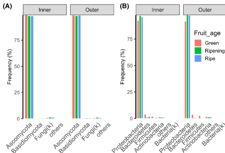
FIGURE 1 The percentage of (A) fungal and (B) bacterial ASVs assigned to each phylum at the 80% confidence level across fruit ages and within-tunnel locations.
