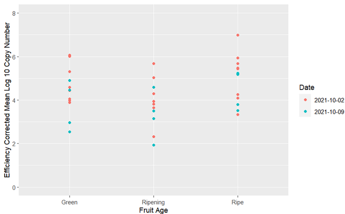
FIGURE A2 The efficiency corrected mean Log 10 copy number quantitative PCR results for the 16S of bacterial epiphytes on the surface of raspberries across fruit ages and two sampling dates.
