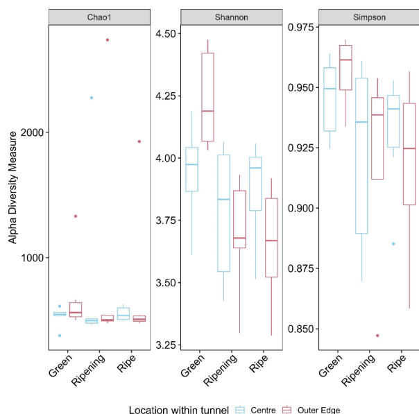
FIGURE 3 The alpha diversity measures for bacterial Amplicon Sequence Variants (ASVs) of Chao1, Shannon and Simpson diversity indices. Four polytunnels were sampled across two repeats in time (2 October 2021 and 9 October 2021). The x-axis denotes fruit ripeness, and the colour denotes location within the polytunnel.
