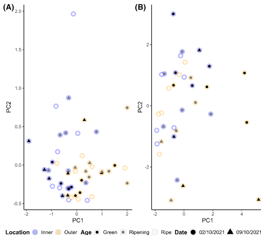
FIGURE A4 The first two principal components for the (A) fungal and (B) bacterial communities on raspberry fruits that were sampled at two time points (2 October 2021 and 9 October 2021), in two locations within polytunnels (centre vs. outer edge) and across three fruit development stages (green, ripening and ripe).
