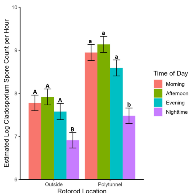
FIGURE 6 The estimated Cladosporium spore counts for samples collected from Rotorod samplers inside a polytunnel and in an open field across the day (morning 08:00–12:00, afternoon 12:00–16:00, evening 16:00–20:00) and the night (20:00–08:00) for 10 days. Letters indicate significant differences between factor levels ( p < 0.05 ).
