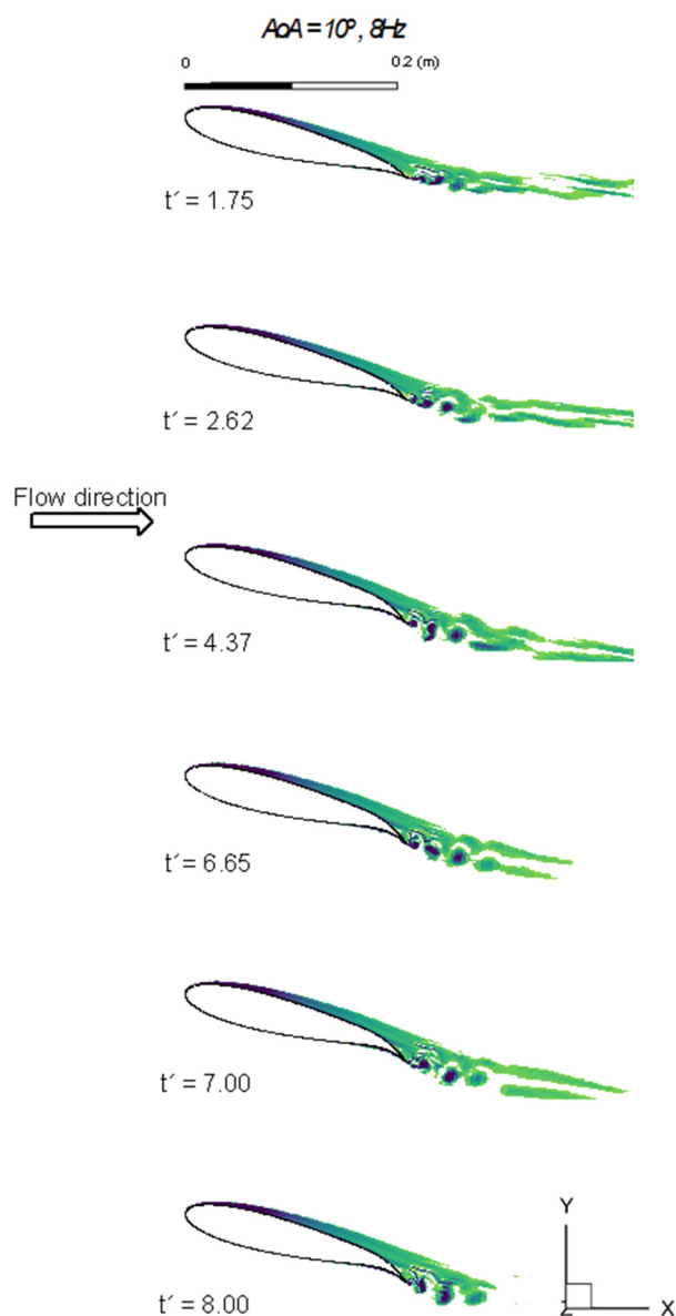
Figure 8. Instantaneous contours of the vorticity showing the evolution of the turbulent structures at AoA = 10^\circ and 8\text{ Hz} .
