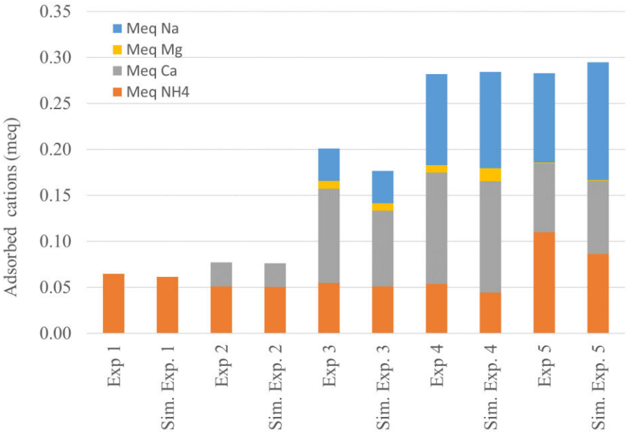
376 Figure 7. Comparison of model results and experimental result under steady-state conditions
