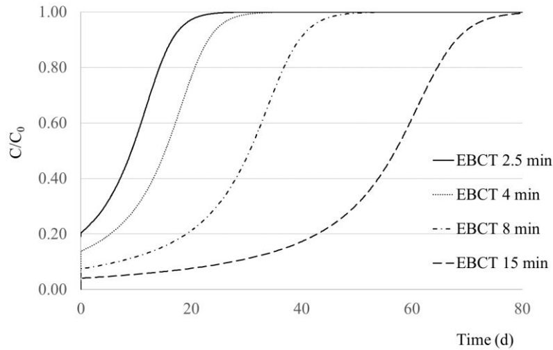
Figure 10. Effect of EBCT on the breakthrough curve
