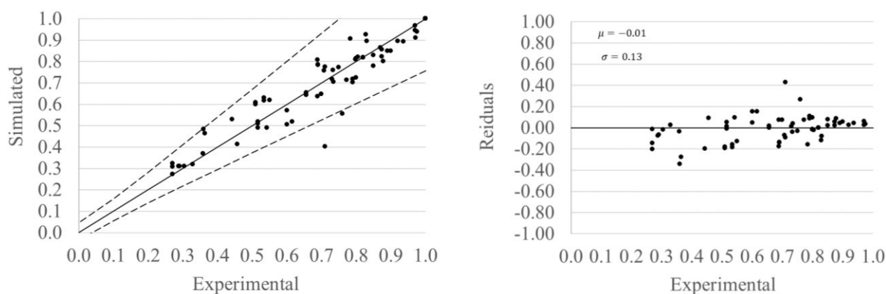
Figure 8. Comparison of experimental and simulated data (Left). The black line represents the linear regression of both sets of data and the dashed lines represent the confidence interval of 95% for the linear regression. Residuals of experimental and simulated data (Right)
