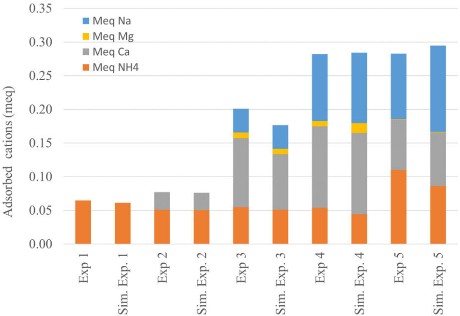
376 Figure 7. Comparison of model results and experimental result under steady-state conditions
