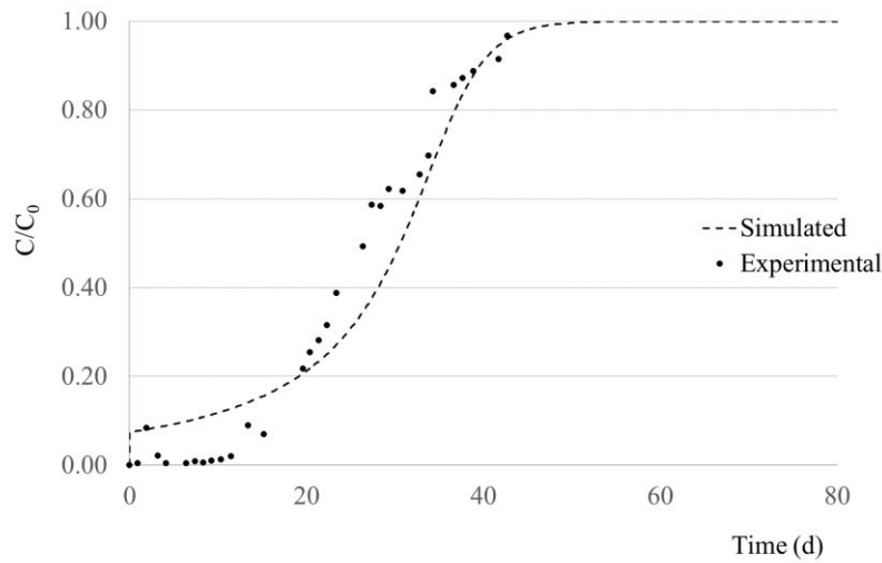
Figure 9. Comparison the experimental and simulated breakthrough curves
