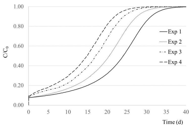
Figure 13. Effect of concentration of competing cations on the breakthrough curve
