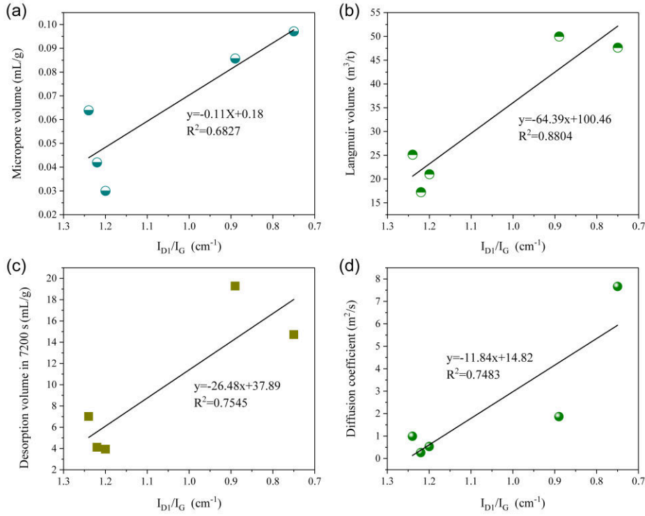
Fig. 11 Relationship between the Raman parameter ( I_{D1}/I_G , intensity ratio of the D peak and the G peak), and micropores volume (a), V_L (b), gas desorption volume within 7200 seconds (c) and D_0 (d)
