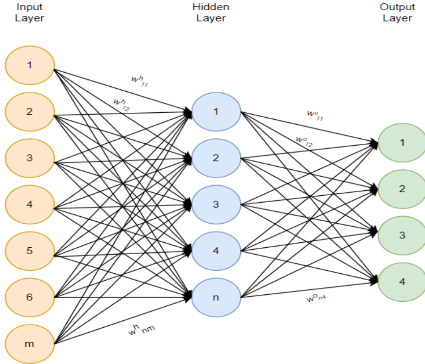
Fig. 3 The FFNN architecture
