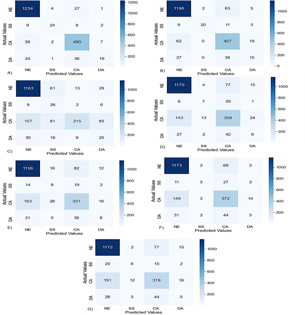
Fig. 10 Confusion matrices for the models after incorporating CS method.
